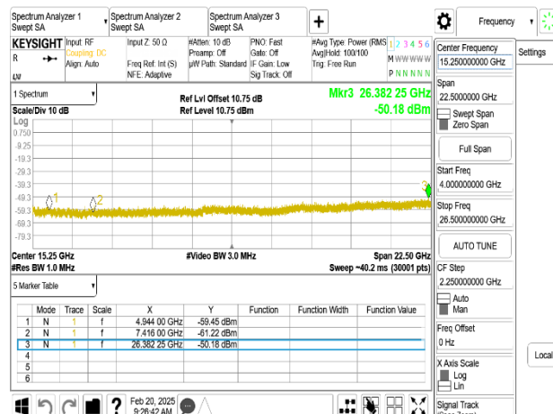
802.11ax_20MHz_Chain0_2472MHz_RU_52_40_4-26.5GHz
