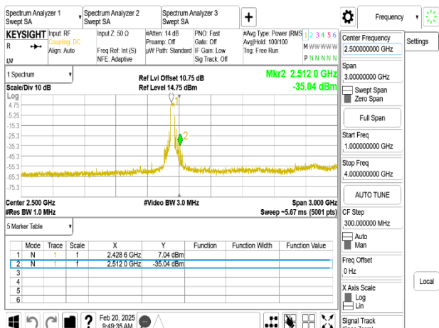
802.11ax_40MHz_Chain0_2437MHz_RU484_1-4GHz
