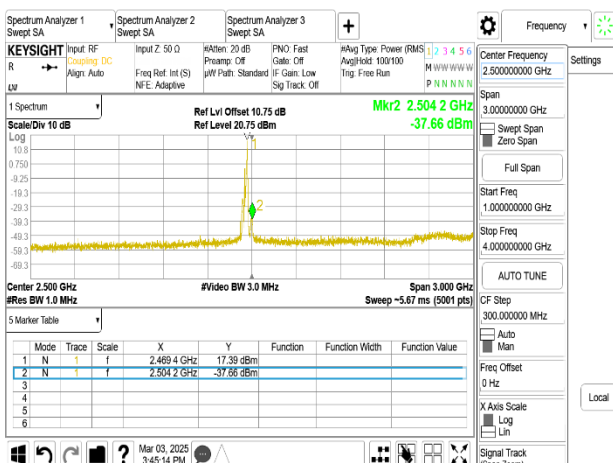
802.11ax_20MHz_Chain0_2462MHz_RU_52_40_1-4GHz
