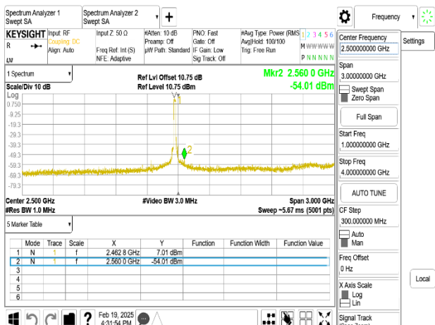
802.11ax_20MHz_Chain0_2467MHz_RU242_1-4GHz
