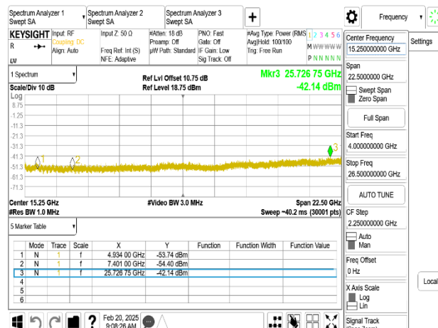
802.11ax_20MHz_Chain0_2467MHz_RU26_8_4-26.5GHz
