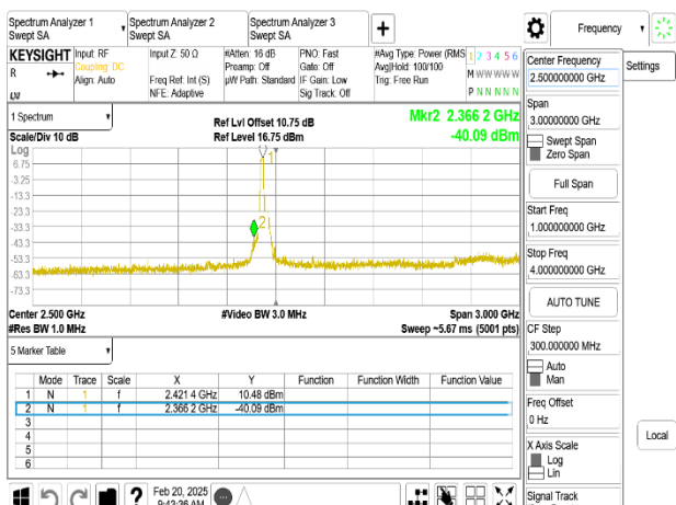
802.11ax_40MHz_Chain0_2422MHz_RU242_61_1-4GHz
