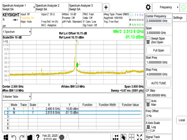
802.11ax_20MHz_Chain0_2472MHz_RU_26_8_1-4GHz
