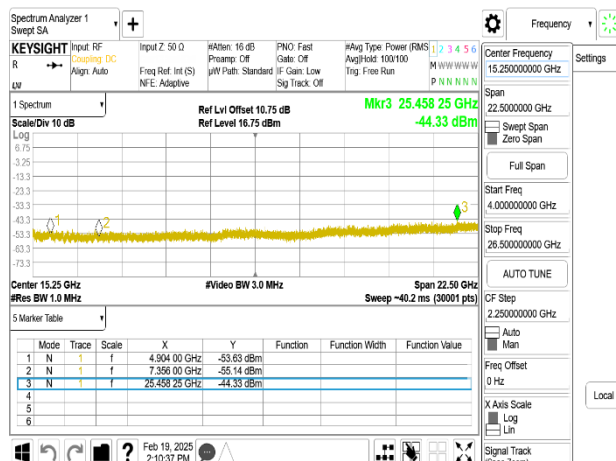
802.11ax_40MHz_Chain0_2452MHz_4-26.5GHz
