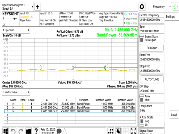
SISO_802.11ax_40MHz_Chain0_2462MHz
