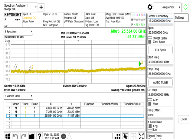
802.11g_20MHz_Chain0_2412MHz_4-26.5GHz
