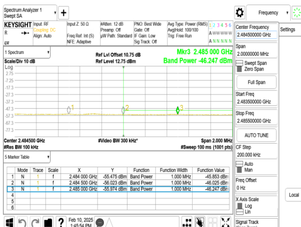
SISO_802.11ax_40MHz_Chain0_2452MHz
