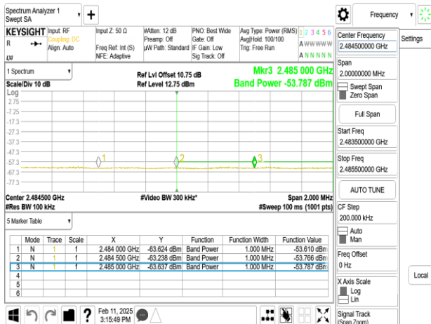
SISO_802.11ax_40MHz_Chain0_2447MHz_RU484
