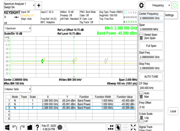
SISO_802.11ax_40MHz_Chain0_2422MHz_RU242_61
