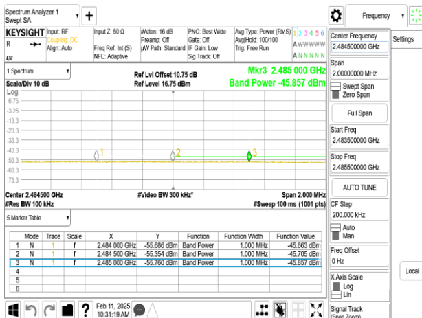
SISO_802.11ax_20MHz_Chain0_2452MHz
