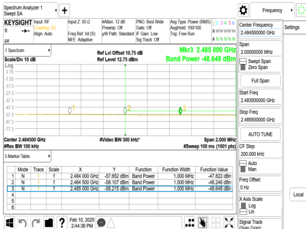
SISO_802.11ax_20MHz_Chain0_2442MHz_RU26_8
