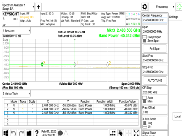
SISO_802.11ax_40MHz_Chain0_2437MHz_RU242_61_L
