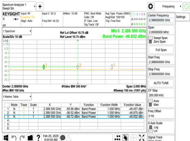
SISO_802.11ax_40MHz_Chain0_2427MHz_RU242_61
