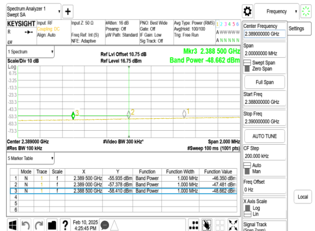
SISO_802.11ax_20MHz_Chain0_2437MHz_RU26_0_L
