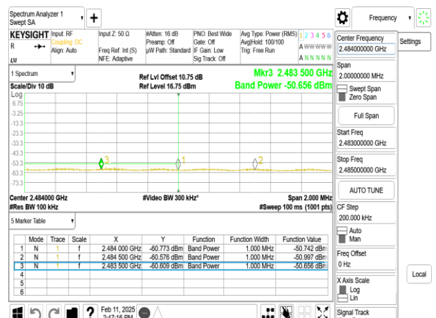
SISO_802.11ax_40MHz_Chain0_2437MHz_RU242_62_R
