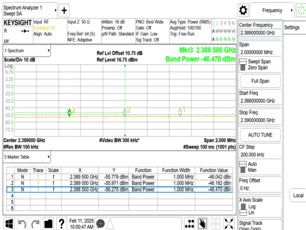
SISO_802.11ax_20MHz_Chain0_2432MHz
