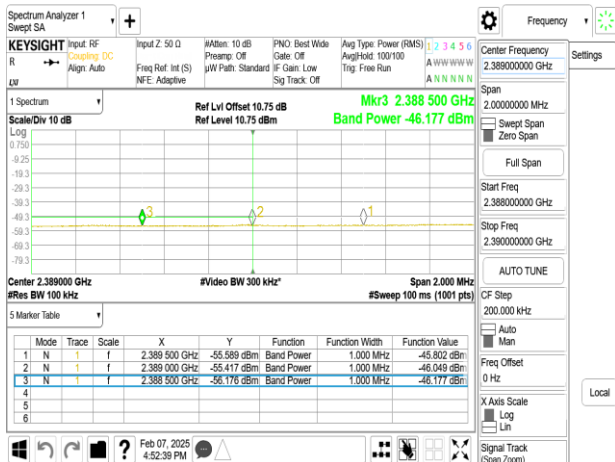
SISO_802.11ax_40MHz_Chain0_2437MHz_R
