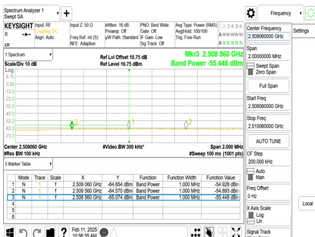
SISO_802.11ax_20MHz_Chain0_2467MHz_RU26_8
