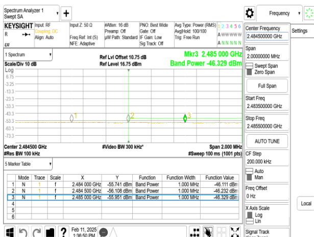
SISO_802.11ax_20MHz_Chain0_2457MHz_RU106_54
