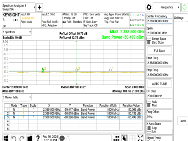
SISO_802.11ax_40MHz_Chain0_2427MHz_RU484
