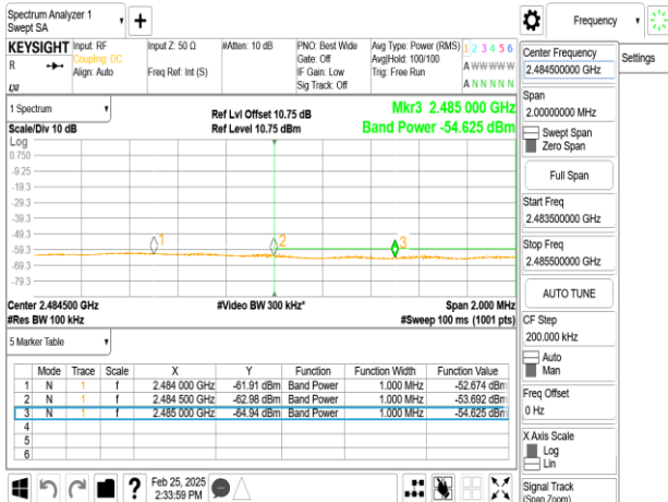
SISO_802.11ax_20MHz_Chain0_2472MHz_RU26_8
