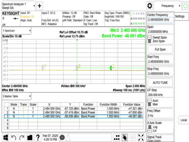
SISO_802.11ax_20MHz_Chain0_2462MHz_RU106_54
