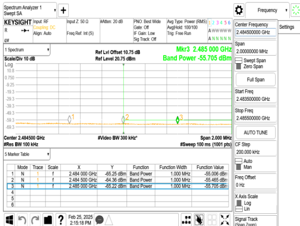
SISO_802.11ax_20MHz_Chain0_2467MHz_RU242
