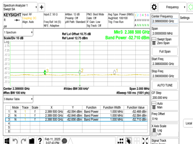
SISO_802.11ax_40MHz_Chain0_2432MHz_RU484
