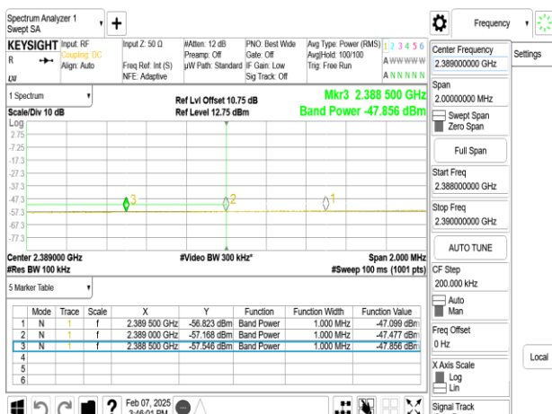
SISO_802.11ax_20MHz_Chain0_2427MHz
