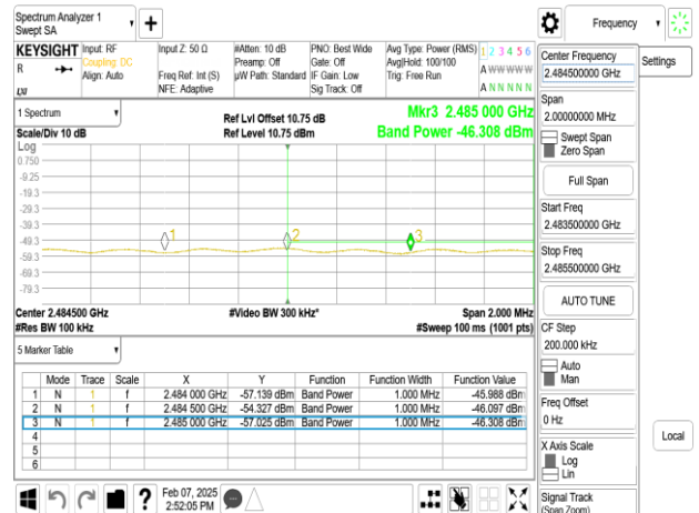
SISO_802.11n_40MHz_Chain0_2462MHz
