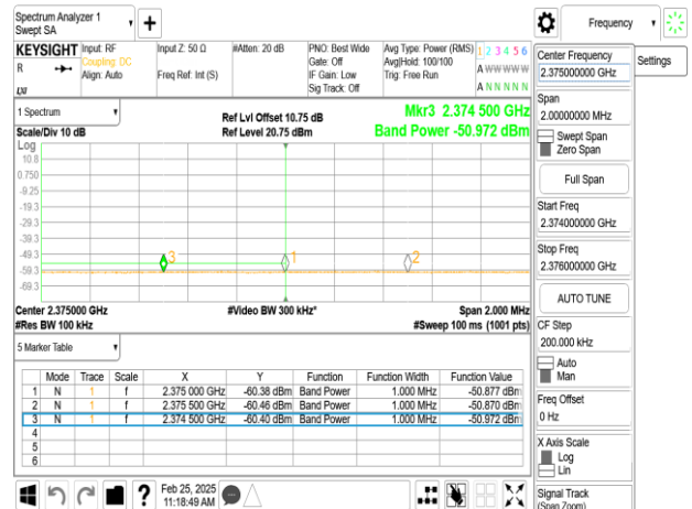
SISO_802.11ax_20MHz_Chain0_2417MHz
