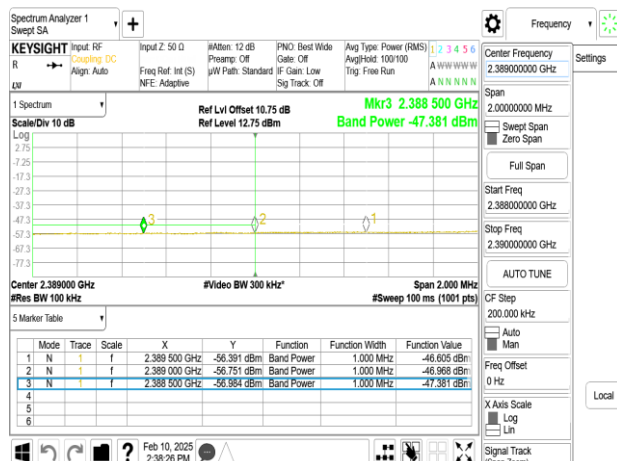
SISO_802.11ax_20MHz_Chain0_2422MHz_RU242
