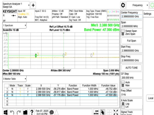
SISO_802.11ax_20MHz_Chain0_2422MHz_RU106_53
