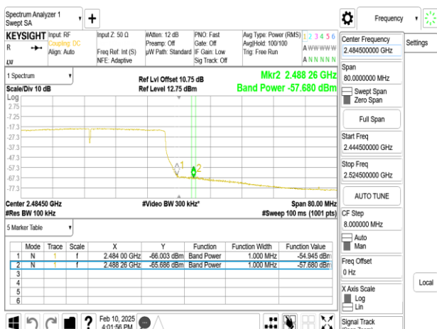
SISO 802.11ax 40MHz Chain0 2462MHz RU484
