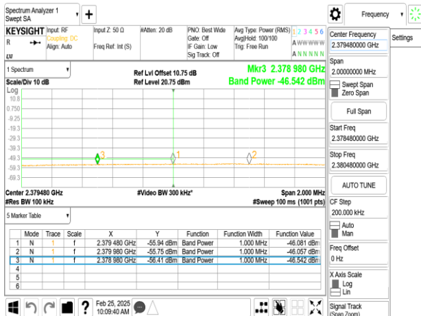
SISO_802.11ax_20MHz_Chain0_2422MHz_RU52_37
