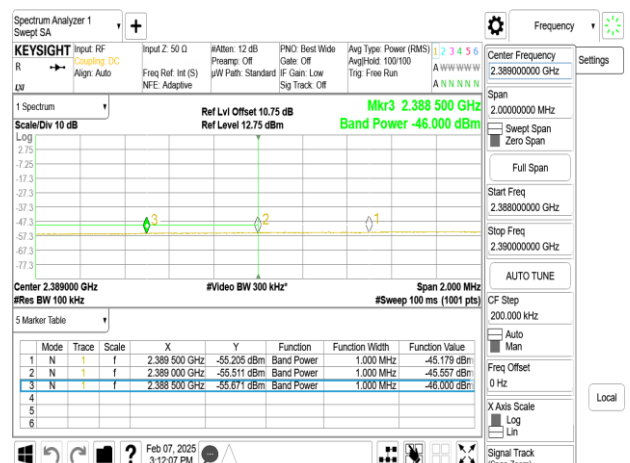
SISO_802.11ax_20MHz_Chain0_2412MHz
