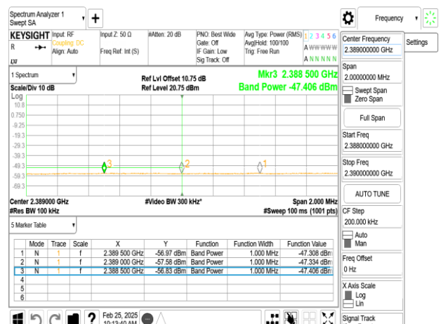
SISO_802.11ax_20MHz_Chain0_2417MHz_RU106_53
