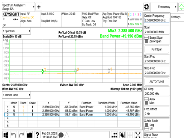
SISO_802.11ax_20MHz_Chain0_2412MHz_RU26_0
