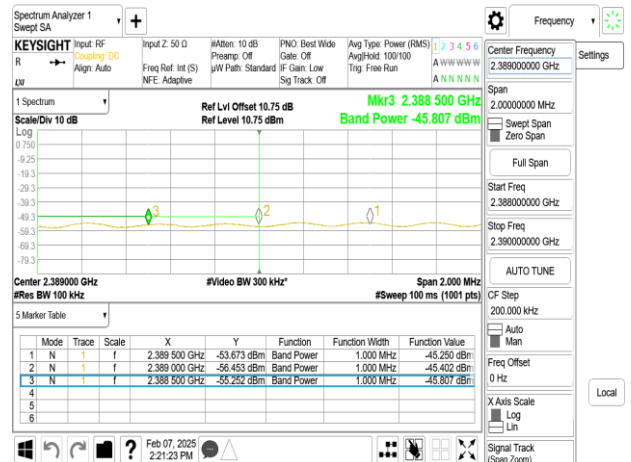
SISO_802.11n_40MHz_Chain0_2432MHz
