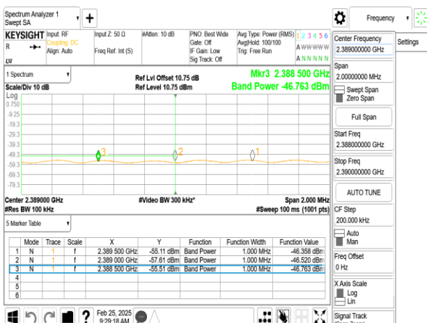
SISO_802.11n_40MHz_Chain0_2422MHz
