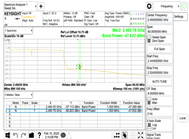
SISO_802.11ax_40MHz_Chain0_2457MHz_RU242_62
