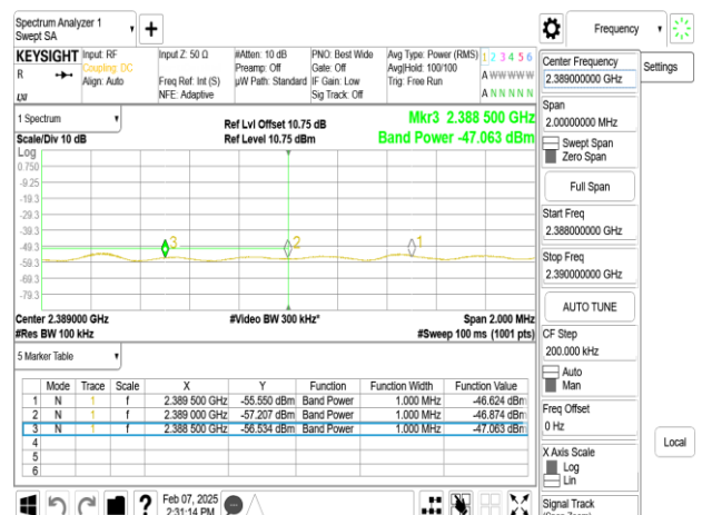
SISO_802.11n_40MHz_Chain0_2437MHz_L
