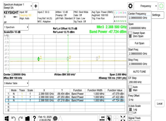
SISO_802.11ax_20MHz_Chain0_2427MHz_RU26_0
