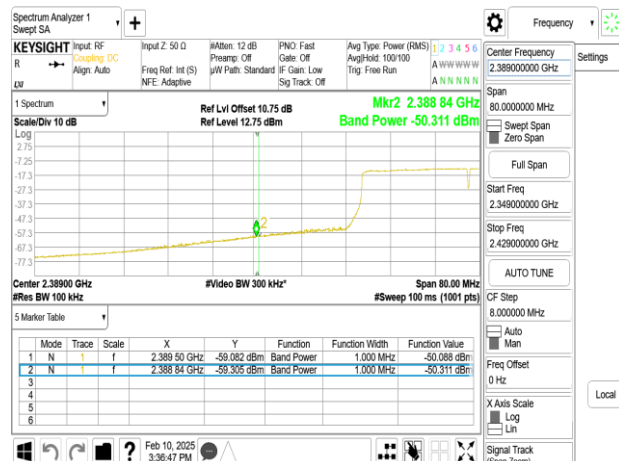
SISO_802.11ax_40MHz_Chain0_2432MHz
