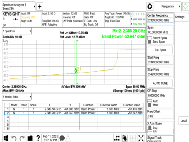
SISO_802.11ax_40MHz_Chain0_2432MHz_RU484
