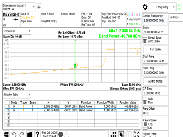
SISO_802.11ax_40MHz_Chain0_2427MHz
