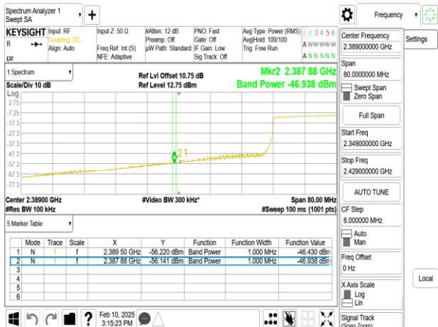
SISO_802.11ax_40MHz_Chain0_2437MHz
