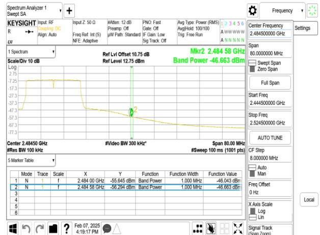
SISO_802.11ax_20MHz_Chain0_2457MHz_RU106_54
