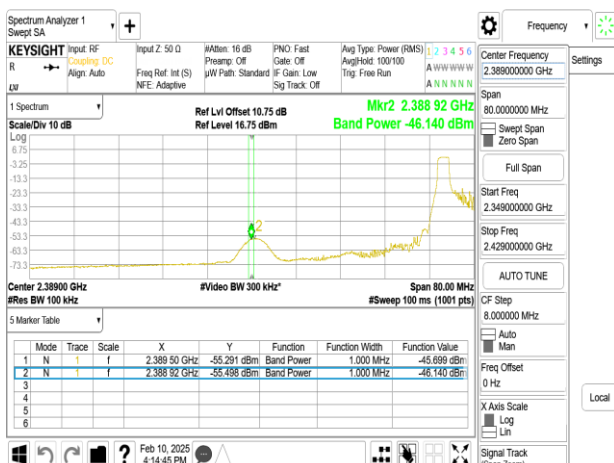
SISO_802.11ax_20MHz_Chain0_2432MHz_RU26_0
