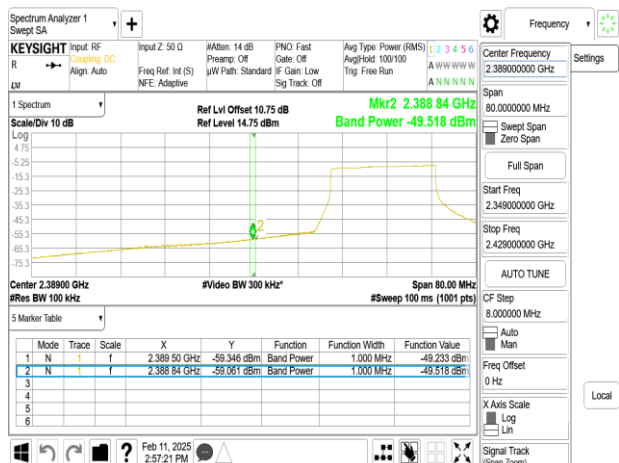
SISO_802.11ax_40MHz_Chain0_2422MHz_RU484
