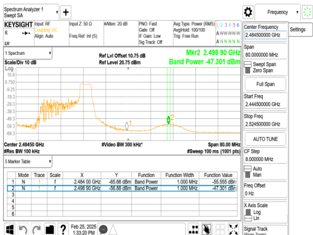
SISO_802.11ax_20MHz_Chain0_2467MHz
