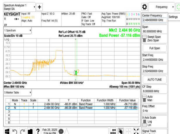
SISO_802.11ax_20MHz_Chain0_2467MHz_RU52_40
