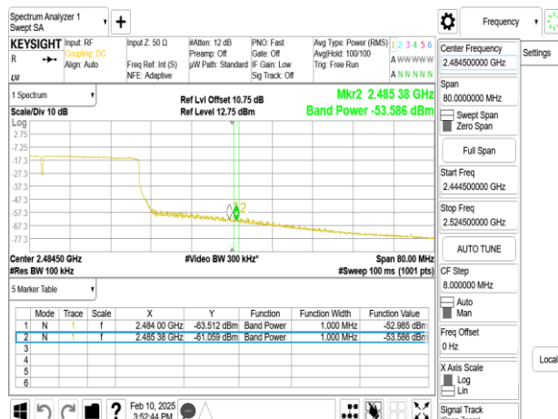
SISO_802.11ax_40MHz_Chain0_2447MHz_RU484
