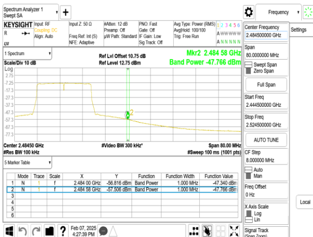
SISO_802.11ax_20MHz_Chain0_2462MHz
