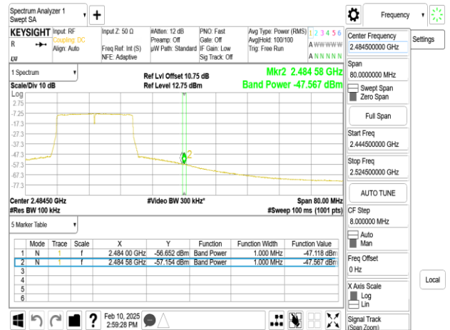
SISO_802.11ax_20MHz_Chain0_2462MHz_RU26_8
