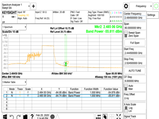
SISO_802.11ax_20MHz_Chain0_2467MHz_RU106_54
