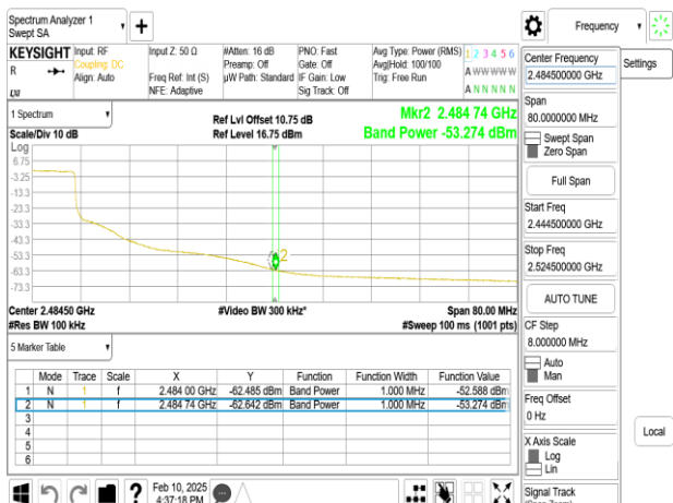
SISO_802.11ax_20MHz_Chain0_2442MHz_RU106_54
