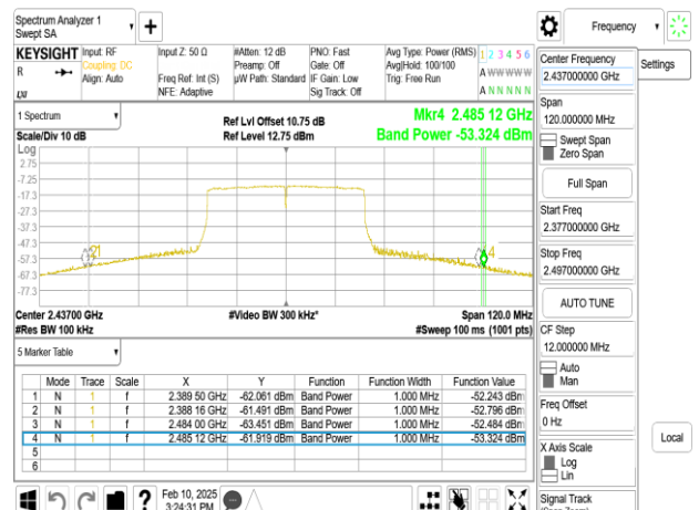
SISO_802.11ax_40MHz_Chain0_2437MHz_RU484
