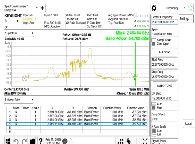
SISO_802.11ax_20MHz_Chain0_2437MHz_RU26_8
