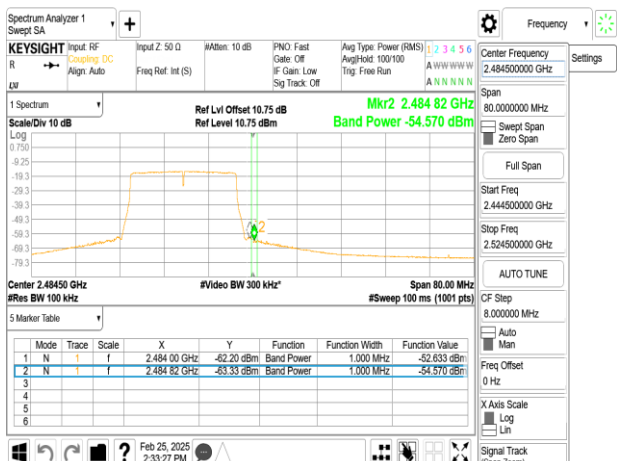
SISO_802.11ax_20MHz_Chain0_2472MHz_RU242
