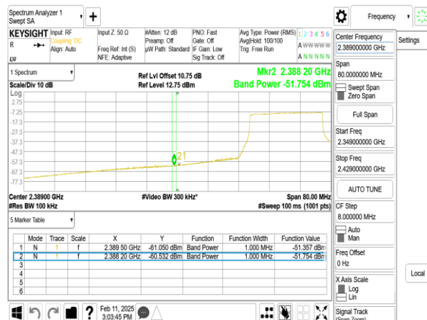
SISO_802.11ax_40MHz_Chain0_2427MHz_RU484
