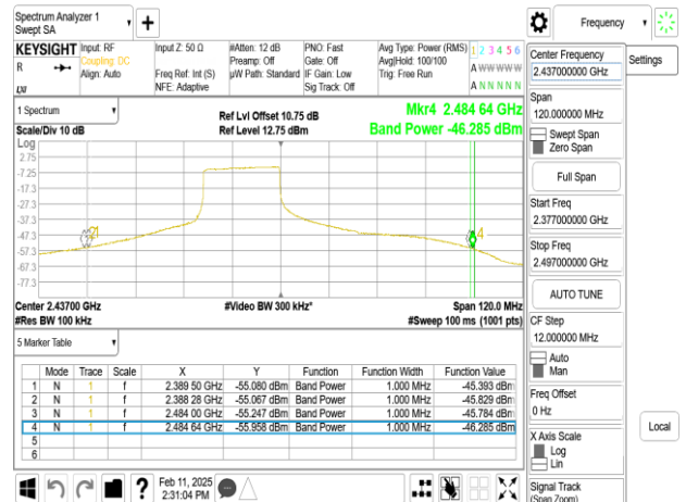
SISO_802.11ax_40MHz_Chain0_2437MHz_RU242_62
