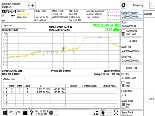
SISO_802.11ax_40MHz_Chain0_2422MHz_RU484
