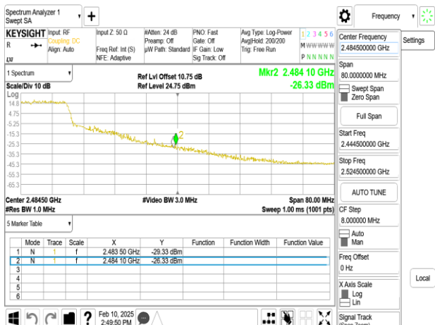
SISO_802.11ax_20MHz_Chain0_2447MHz_RU26_8
