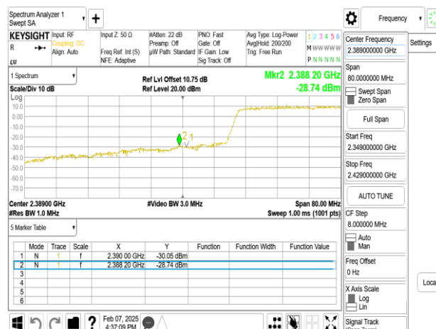
SISO_802.11ax_40MHz_Chain0_2422MHz
