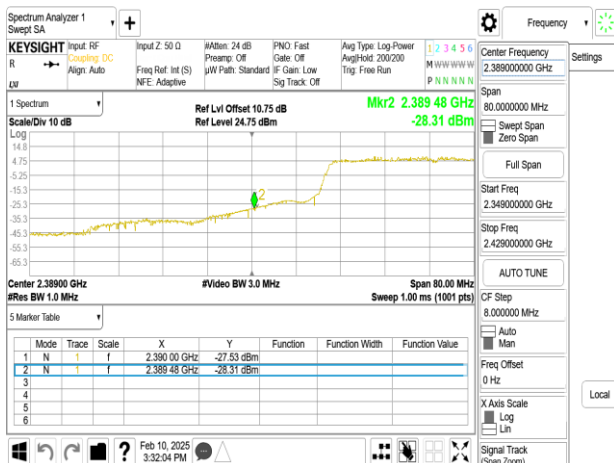
SISO_802.11ax_40MHz_Chain0_2427MHz
