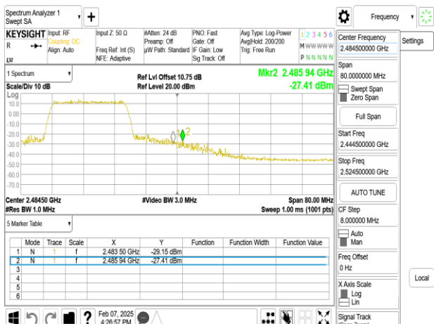
SISO_802.11ax_20MHz_Chain0_2462MHz
