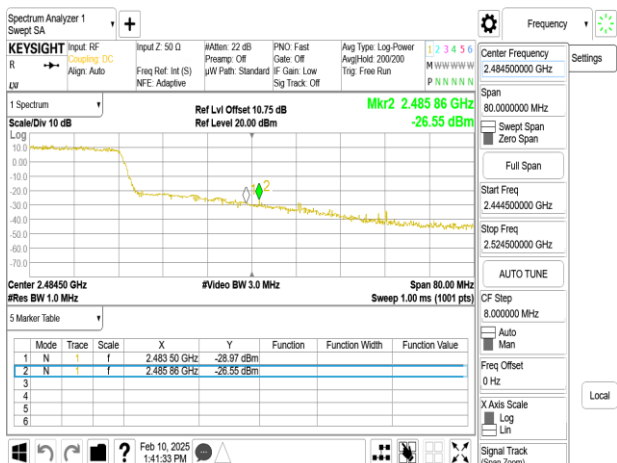
SISO_802.11ax_40MHz_Chain0_2442MHz_RU242_62
