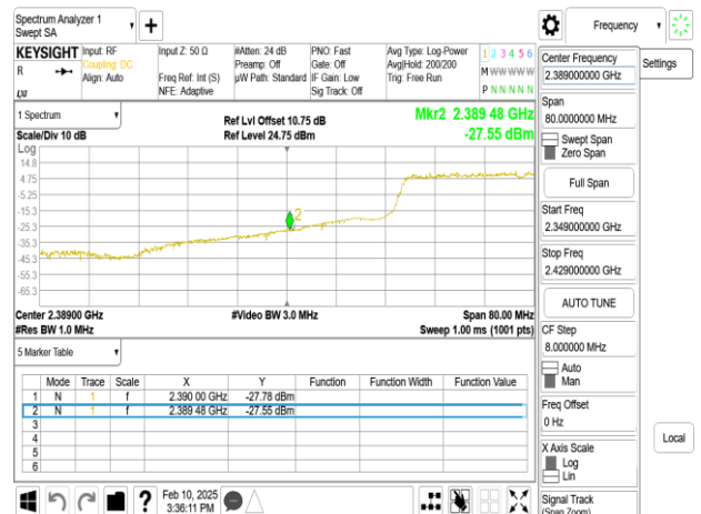
SISO_802.11ax_40MHz_Chain0_2432MHz
