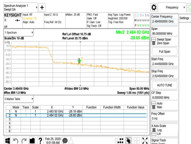
SISO_802.11ax_40MHz_Chain0_2447MHz_RU242_62
