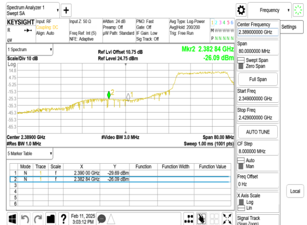
SISO_802.11ax_40MHz_Chain0_2427MHz_RU484
