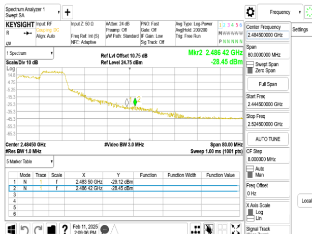
SISO_802.11ax_20MHz_Chain0_2452MHz_RU106_54
