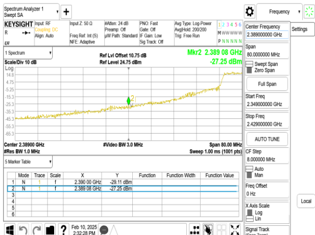
SISO_802.11ax_20MHz_Chain0_2432MHz_RU26_0
