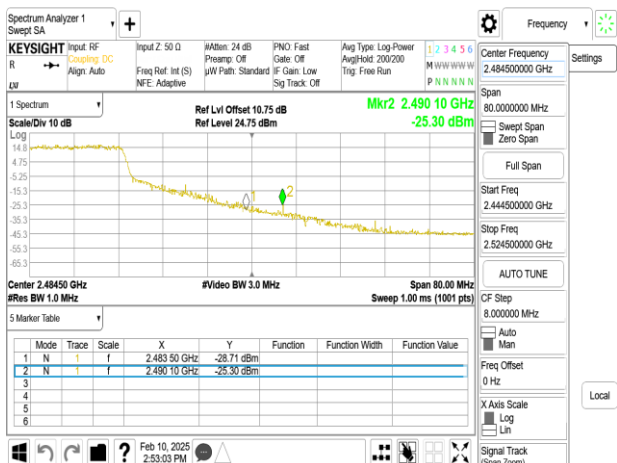
SISO_802.11ax_20MHz_Chain0_2452MHz_RU26_8
