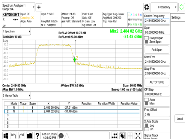
SISO_802.11ax_20MHz_Chain0_2472MHz_RU106_54
