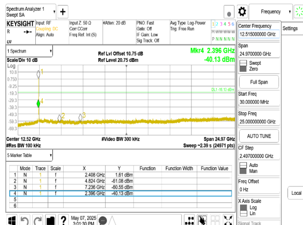
802.11ax_20MHz_Chain0_2412MHz_RU106_53
