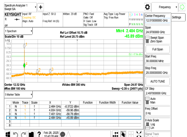
802.11ax_20MHz_Chain0_2467MHz
