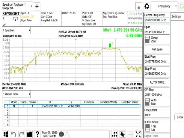
802.11ax_20MHz_Chain0_2472MHz_RU106_54
