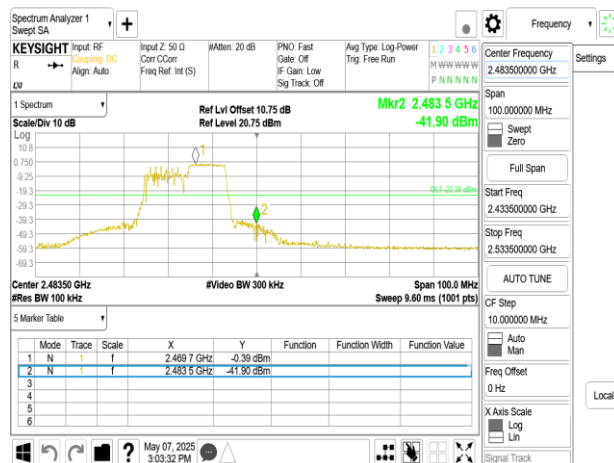
802.11ax_20MHz_Chain0_2467MHz_RU242
