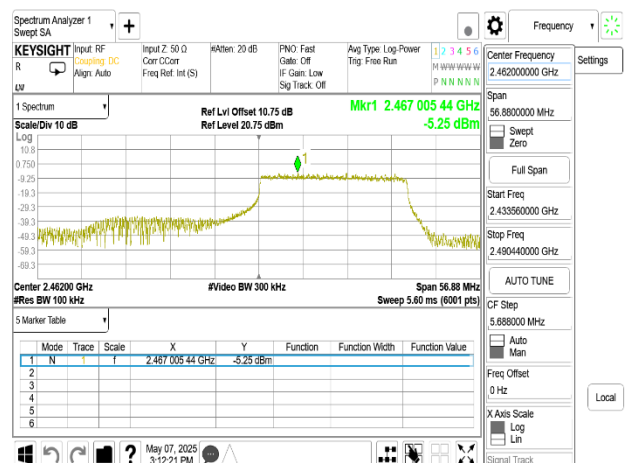
802.11ax_40MHz_Chain0_2462MHz_RU242_62
