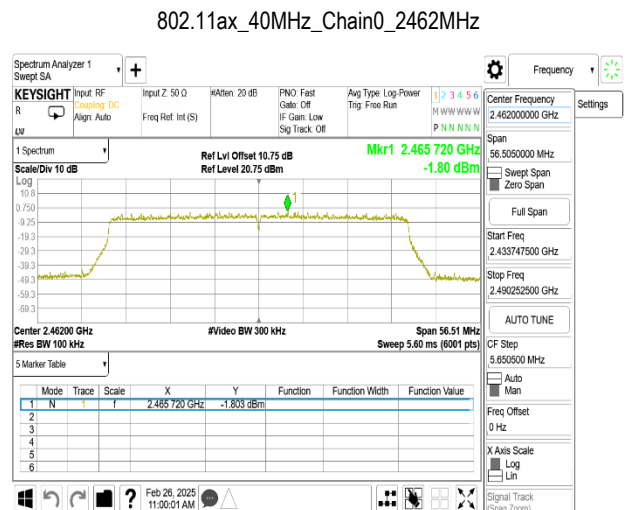
802.11ax_40MHz_Chain0_2462MHz_RU242_62
