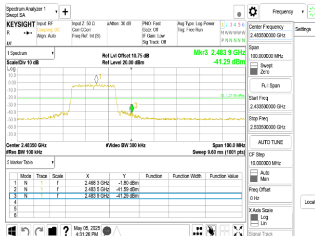
802.11ax_20MHz_Chain0_2467MHz_RU26_8
