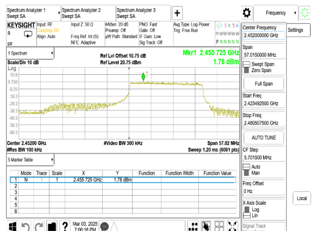
802.11ax_40MHz_Chain0_2452MHz_RU242_62
