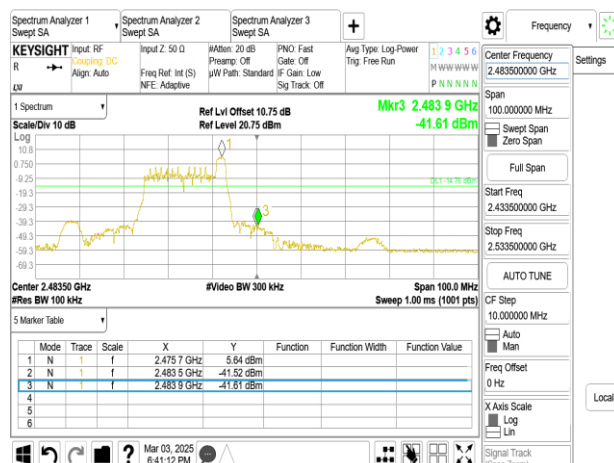
802.11ax_20MHz_Chain0_2467MHz_RU26_8
