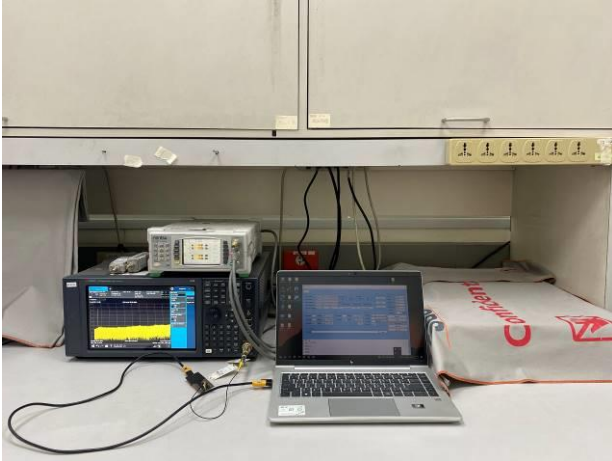
FCC_15_247_Thread_Conducted_Setup
