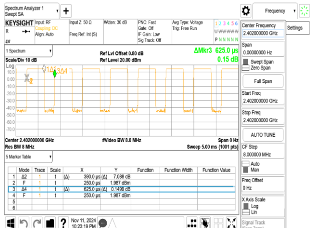
BLE_2M_LowCH00-2402
