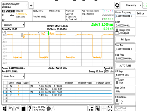
Dwell Time_8DPSK_3M_DH5_2441MHz
