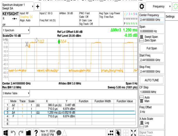
Dwell Time_8DPSK_3M_DH3_2441MHz
