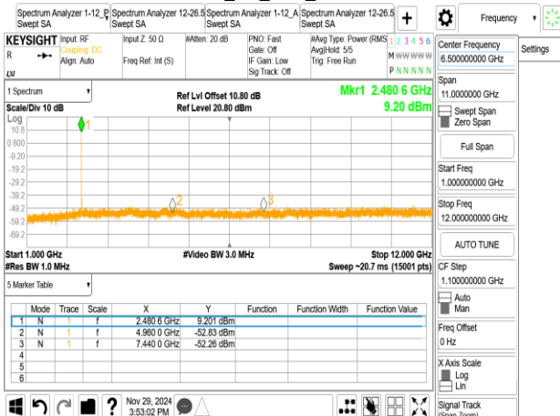
GFSK_1M_DH5_2480MHz
