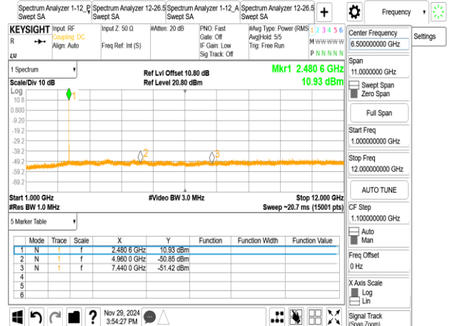
8DPSK_3M_DH5_2480MHz
