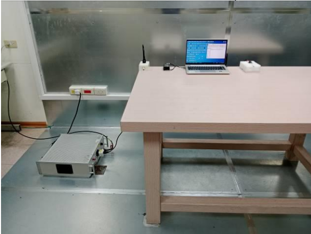
FCC_15_247_BT_Conduction_Setup
