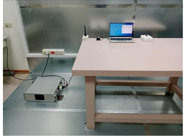
FCC_15_247_Thread_Conduction_Setup
