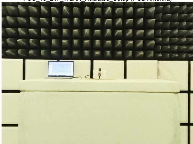
FCC_15_247 WLAN Radiated Setup (PCB Antenna)
