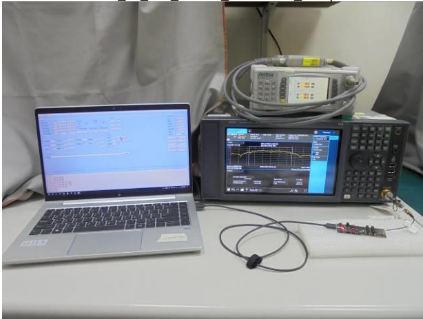
FCC_15_247_Thread_Conducted_Setup
