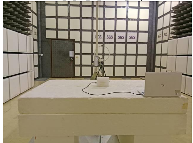
FCC 15 247 BT Radiated Setup
