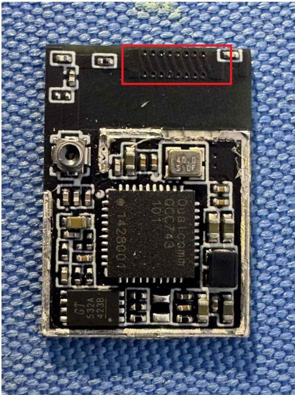
PCB Antenna
