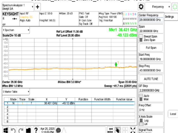
802.11a_20MHz_Chain0_5745MHz_18-40GHz
