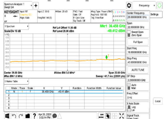
802.11n_20MHz_Chain0_5825MHz_18-40GHz
