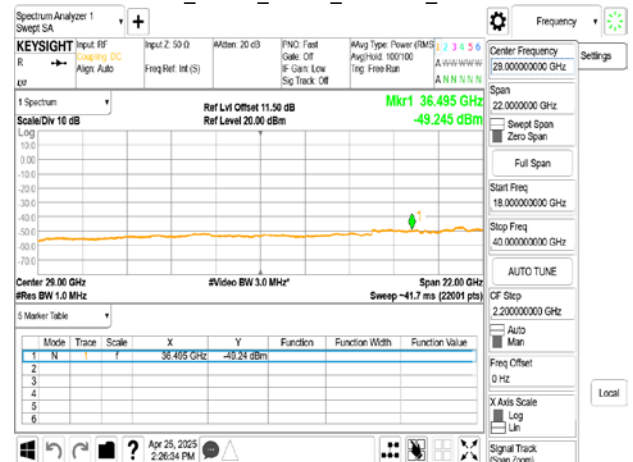
802.11n_20MHz_Chain0_5500MHz_18-40GHz
