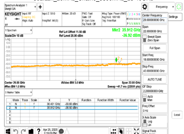
802.11n_20MHz_Chain0_5300MHz_18-40GHz
