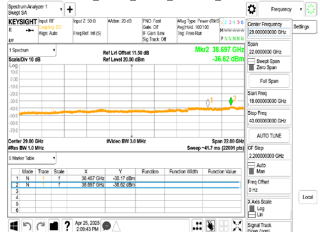
802.11n_20MHz_Chain0_5240MHz_18-40GHz
