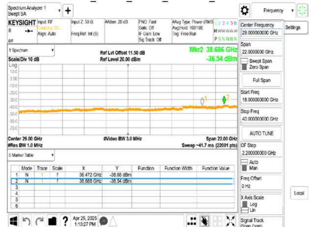
802.11a_20MHz_Chain0_5720MHz_18-40GHz
