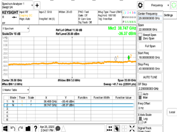
802.11n_20MHz_Chain0_5220MHz_18-40GHz
