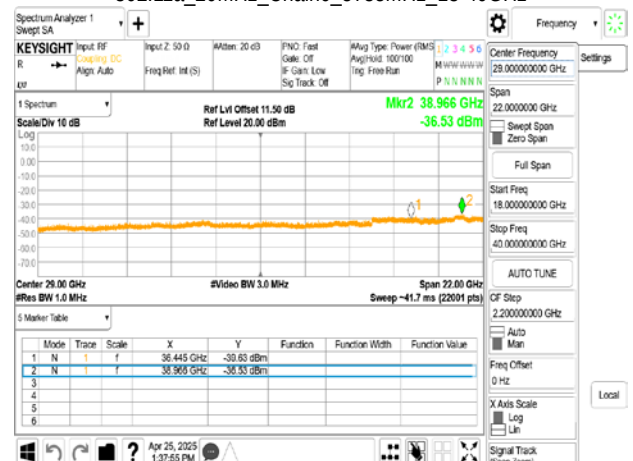
802.11a_20MHz_Chain0_5785MHz_18-40GHz
