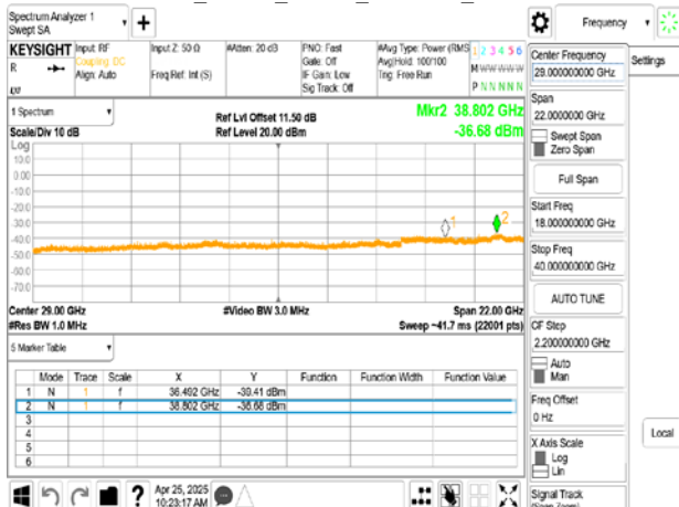
802.11a_20MHz_Chain0_5180MHz_18-40GHz
