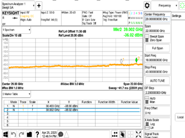
802.11a_20MHz_Chain0_5300MHz_18-40GHz
