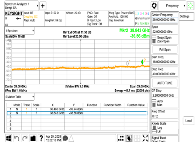
802.11a_20MHz_Chain0_5320MHz_18-40GHz
