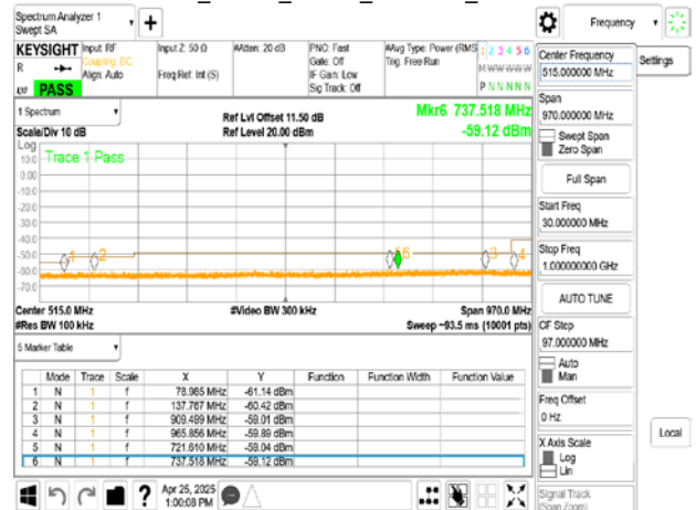
802.11a_20MHz_Chain0_5785MHz_0.03-1GHz
