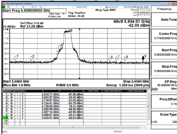
SISO 802.11n 20MHz Chain0 5745MHz
