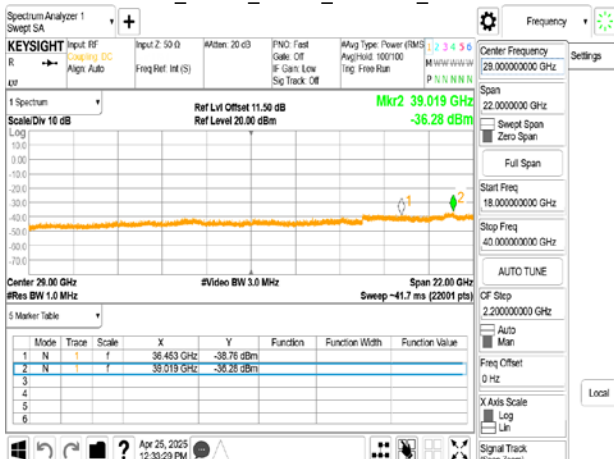
802.11a_20MHz_Chain0_5240MHz_18-40GHz
