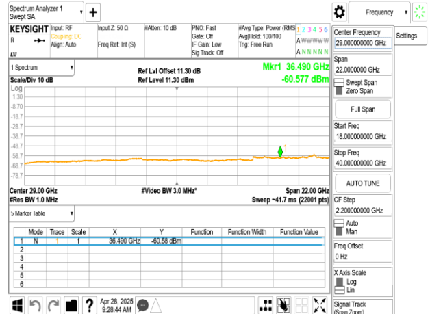
802.11a_20MHz_Chain0_5580MHz_18-40GHz
