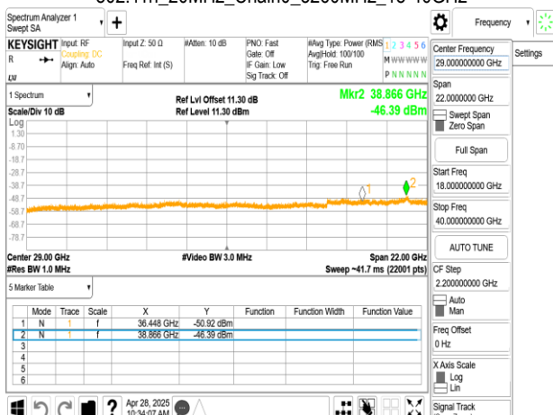
802.11n_20MHz_Chain0_5260MHz_18-40GHz
