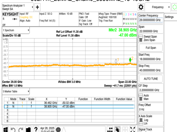
802.11n_20MHz_Chain0_5580MHz_18-40GHz
