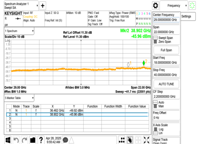
802.11a_20MHz_Chain0_5785MHz_18-40GHz
