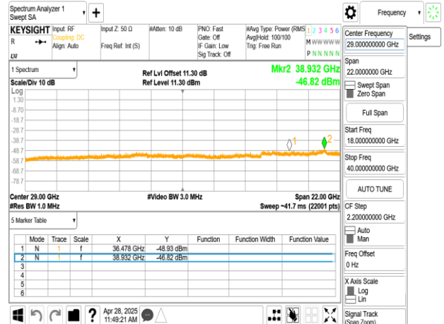
802.11n_20MHz_Chain0_5745MHz_18-40GHz
