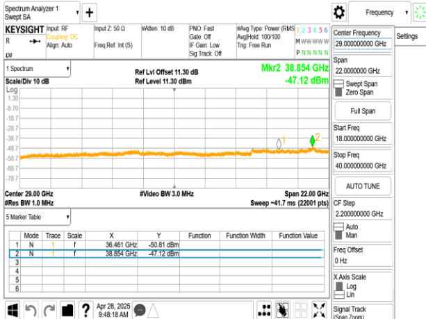
802.11a_20MHz_Chain0_5745MHz_18-40GHz
