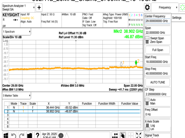
802.11a_20MHz_Chain0_5700MHz_18-40GHz
