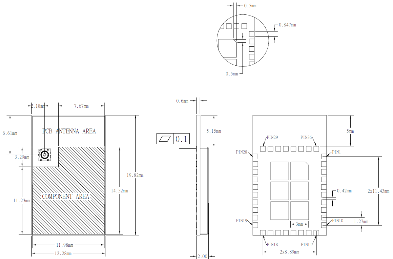
Figure 6: CQM730i-1B Module Dimension
