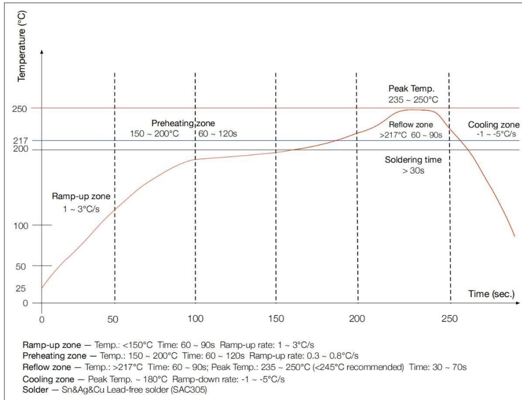
Figure 9: Soldering Guideline
