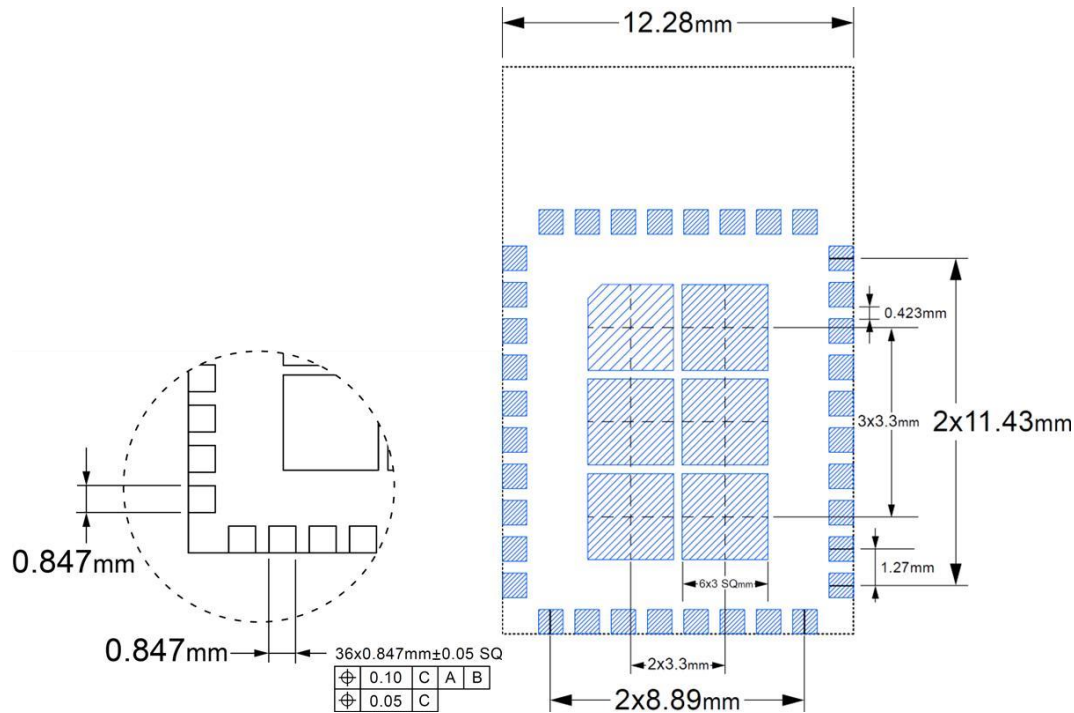
Figure 7: CQM730i-1B Module PCB Landing Pattern
