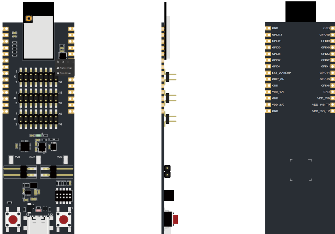
Figure 2: CQM730-1 Module Development Kit
