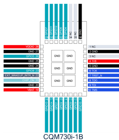
Figure 4: CQM730i-1 Module Pin Map
