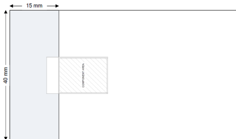
Figure 8: RF Layout Guideline
