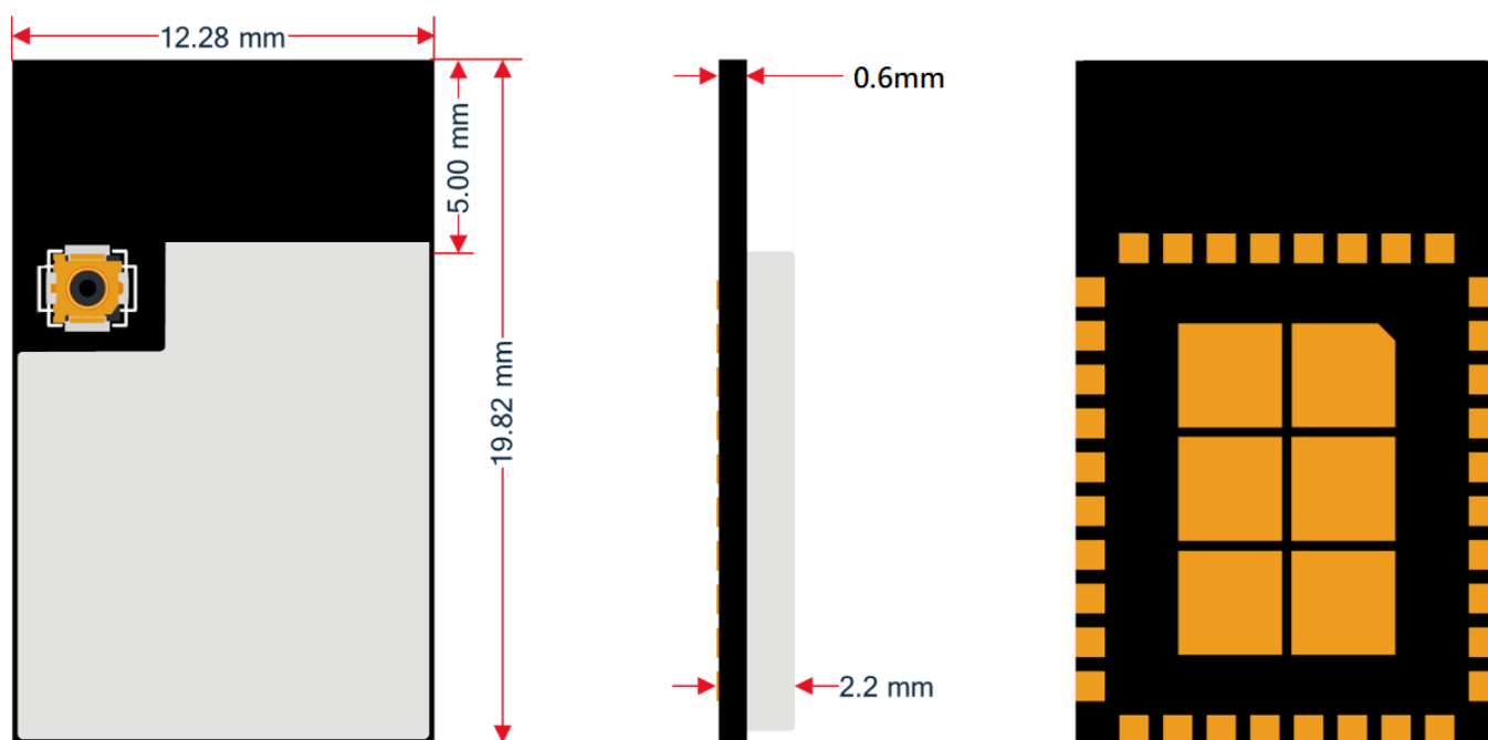
Figure 1: CQM730i-1B Module View
