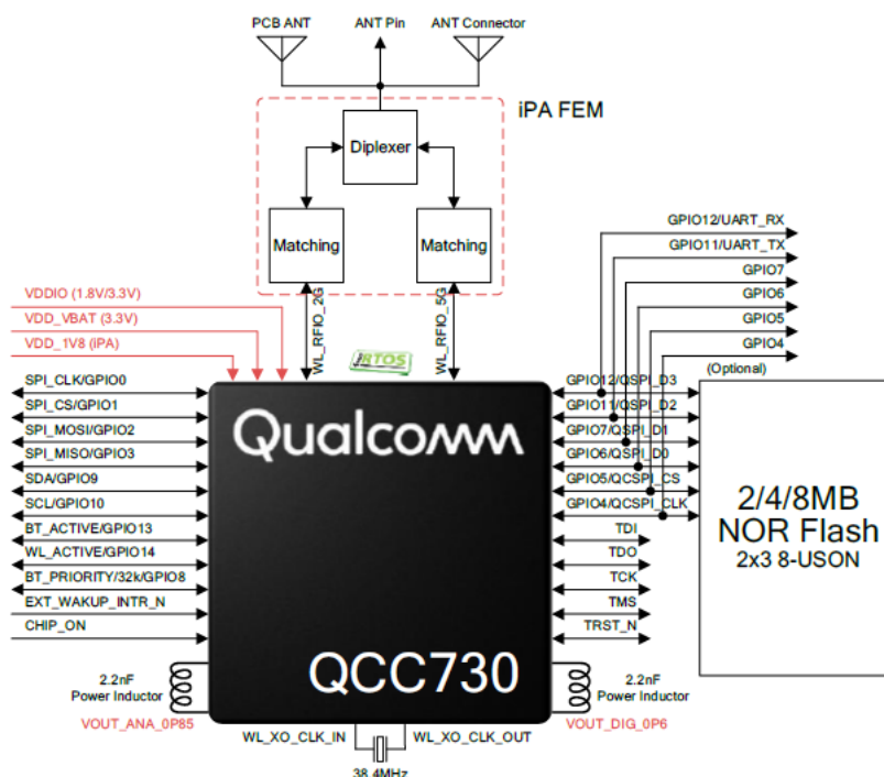
Figure 3: CQM730i-1 Module Block Diagram
