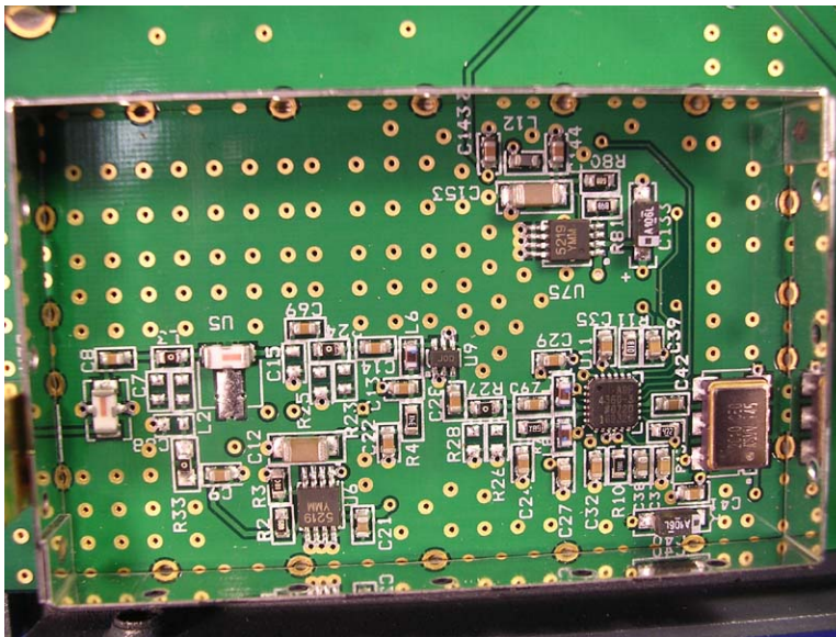
Transmitter Section
