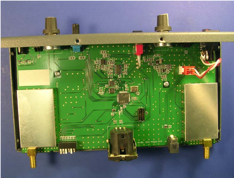
EUT Exposed
