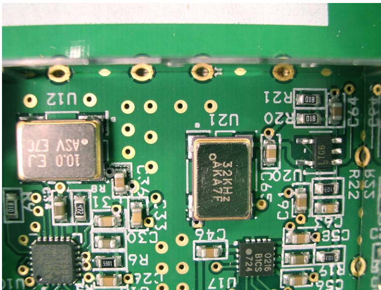
Receiver xtal
