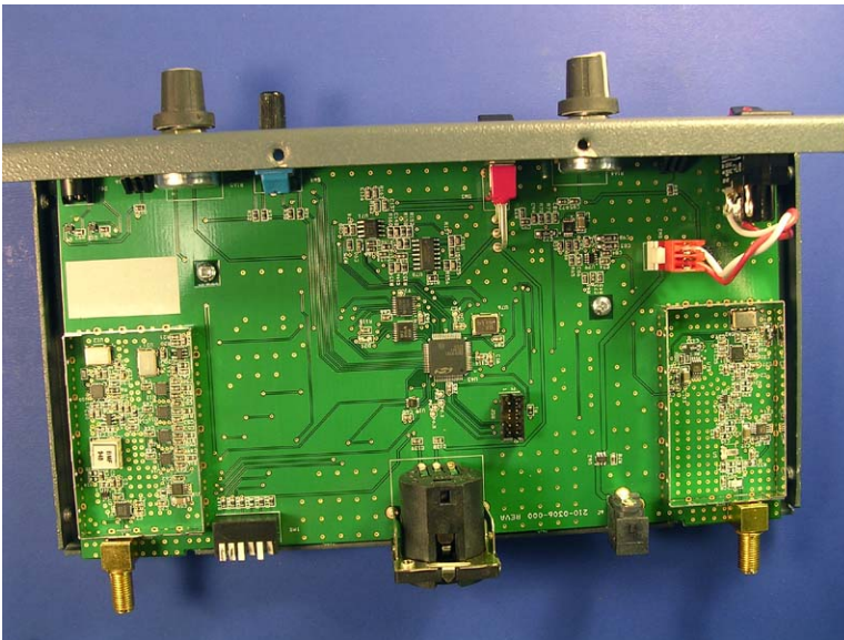
EUT Exposed RF Shield Removed
