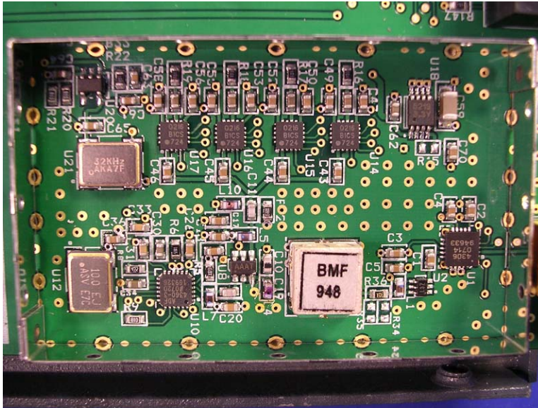
Receiver Section
