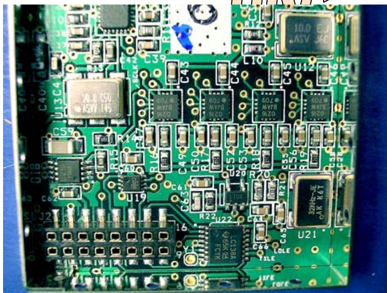
RF PCB 1
