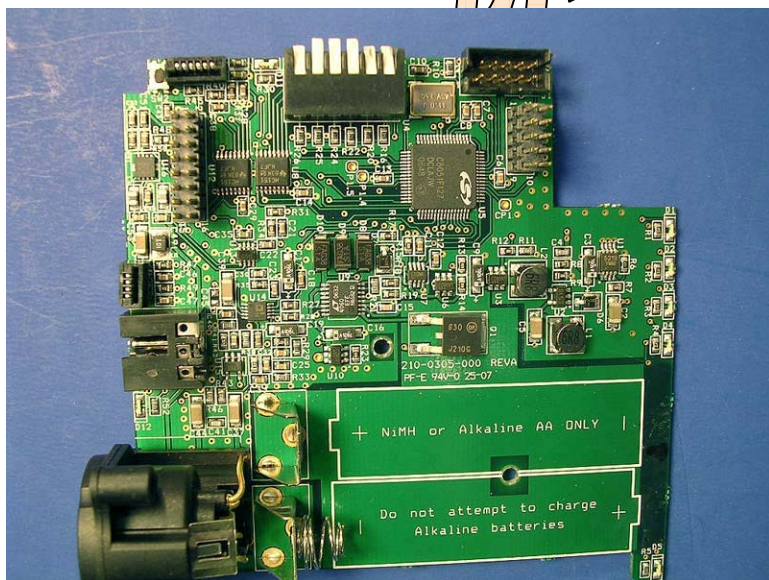
Control PCB
