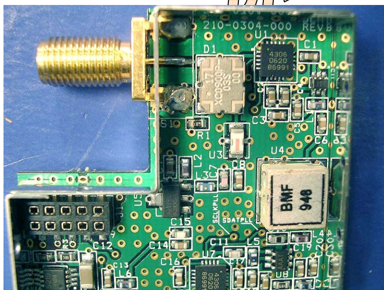
RF PCB 3
