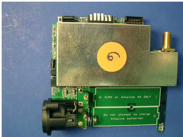
PCB 2
