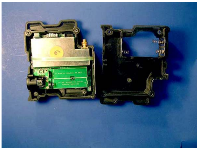
EUT Opened
