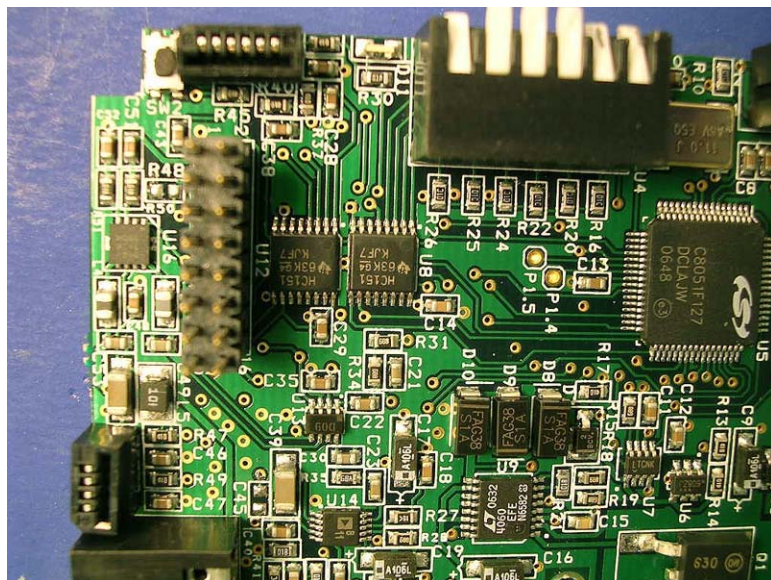
Control PCB 2
