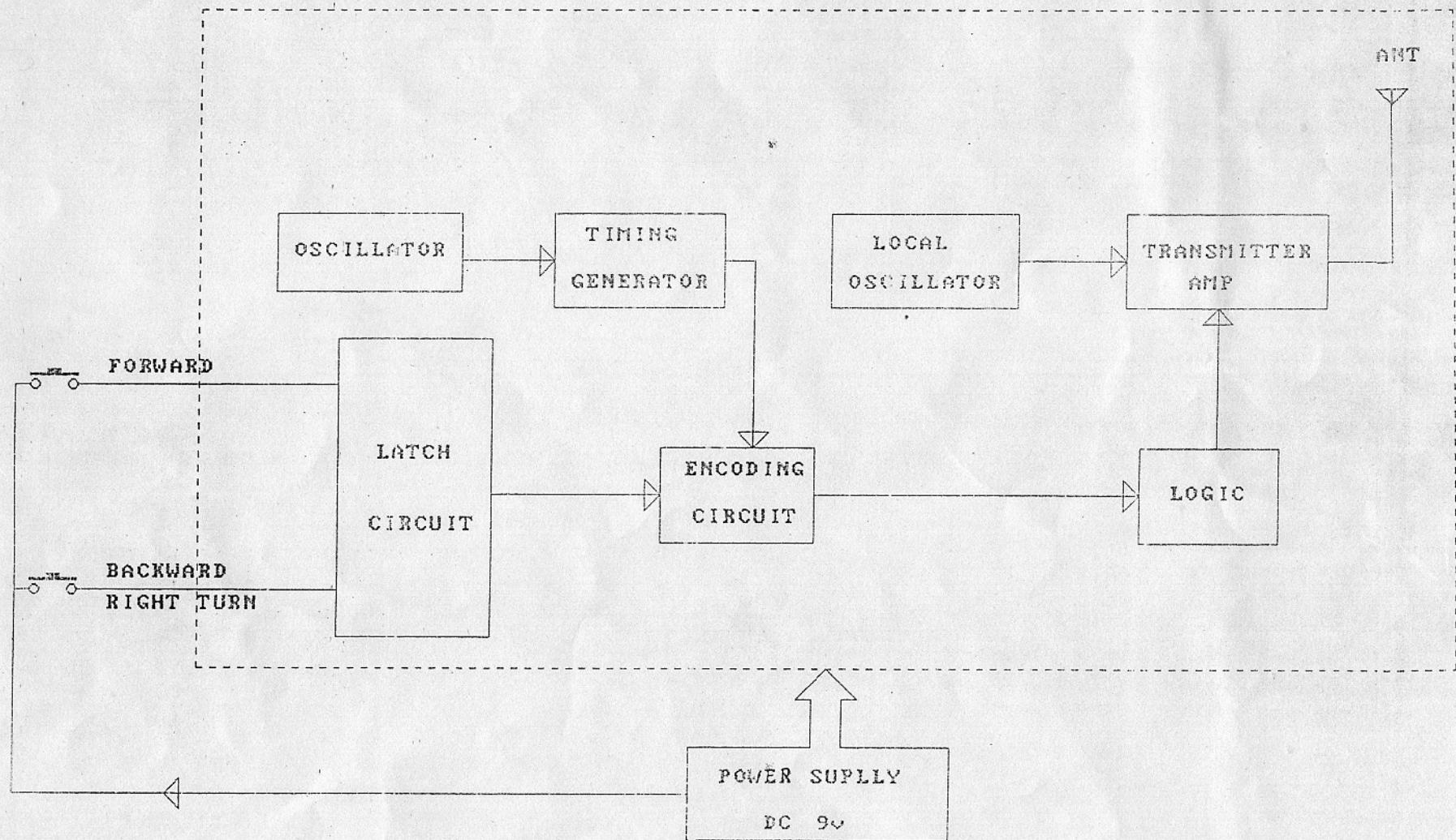
BLOCK DIAGRAM
