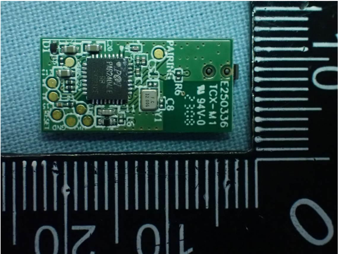
Figure 11 PCB, Back View
