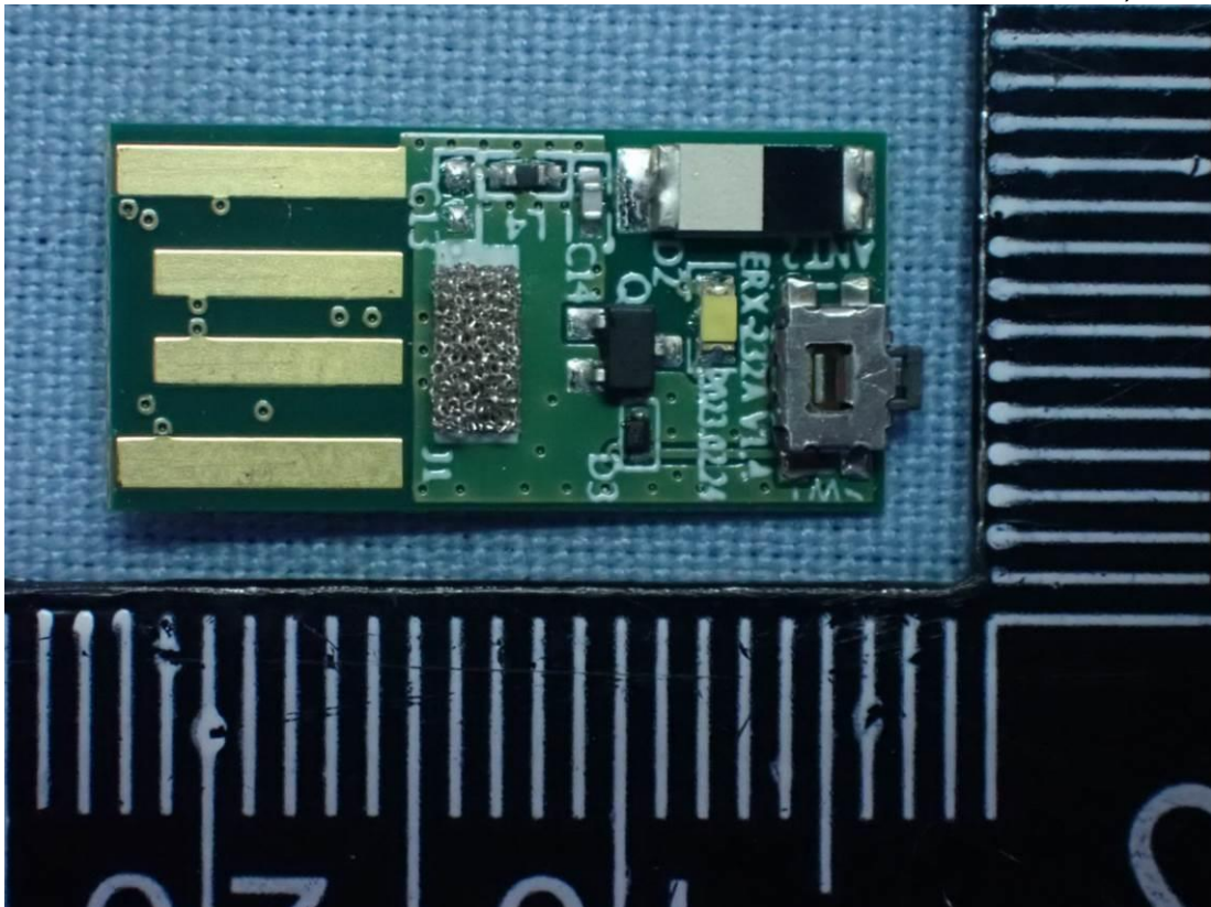
Figure 10 PCB, Front View
