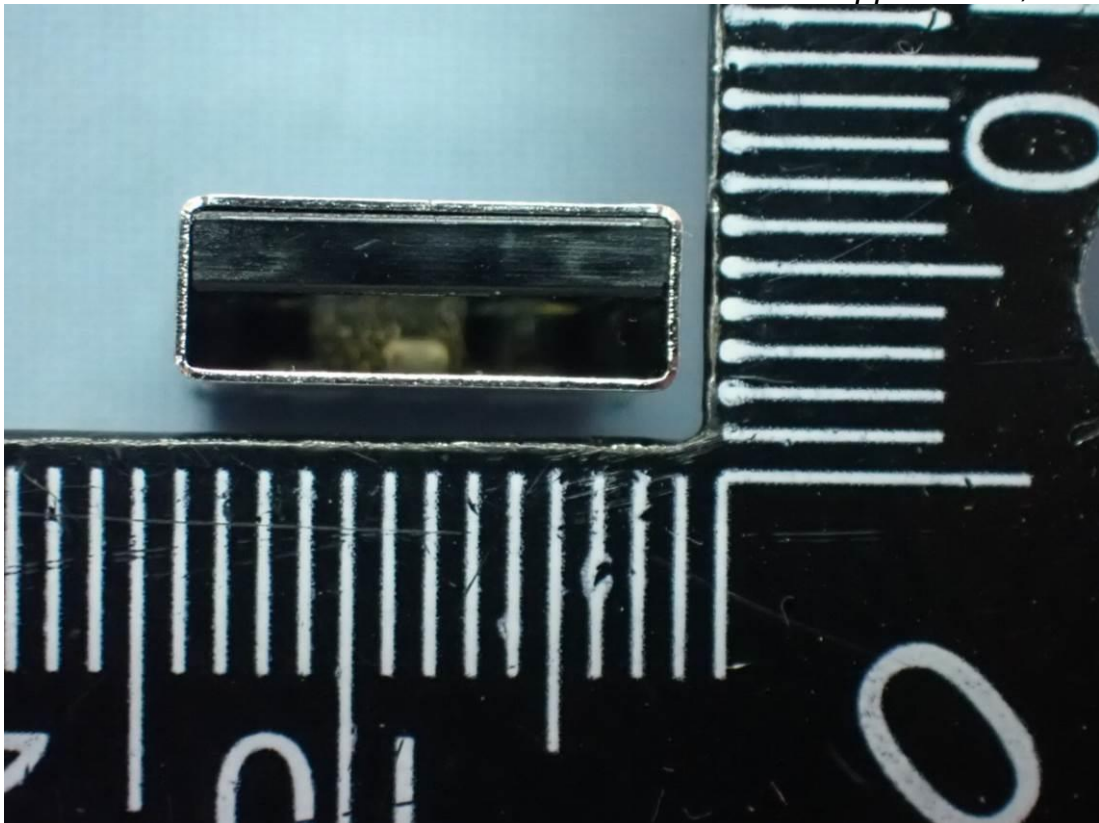
Figure 6 General Appearance, Front View
