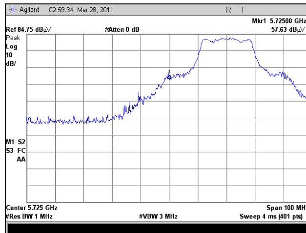
Plot 137. EIRP, 802.11n 20 MHz, 5725 MHz, Peak
