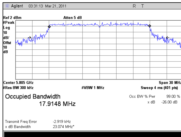
Plot 17. 26 dB Occupied Bandwidth, 802.11n 20 MHz, Port 1, High Channel
