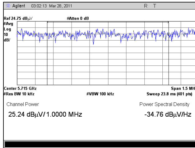
Plot 136. EIRP, 802.11n 20 MHz, 5715 MHz
