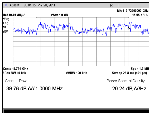
Plot 138. EIRP, 802.11n 20 MHz, 5725 MHz
