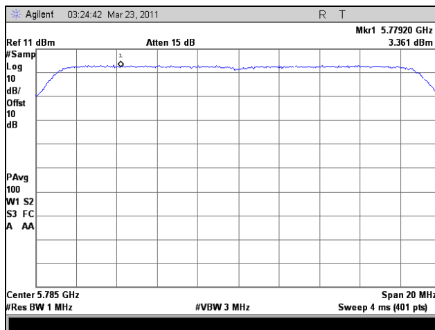
Plot 55. PPSD, 802.11n 20 MHz, Port 1, Mid Channel
