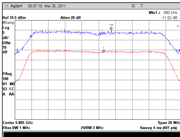
Plot 63. Peak Excursion, 802.11a, High Channel
