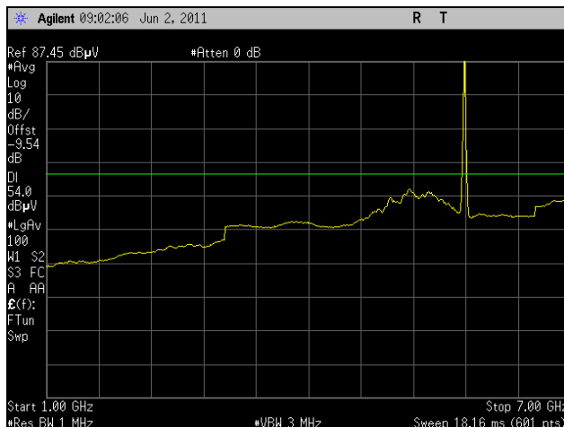
Plot 103. Radiated Spurious Emissions, 802.11n 20 MHz, Mid Channel, 1 GHz – 7 GHz, Average
