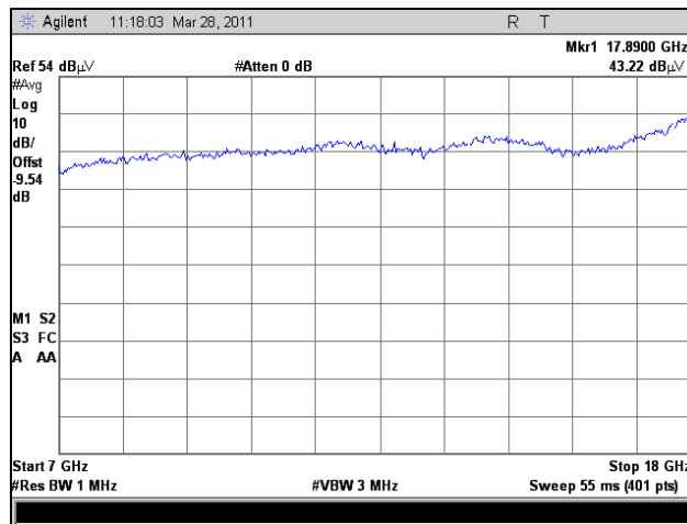
Plot 119. Radiated Spurious Emissions, 802.11n 40 MHz, Low Channel, 7 GHz – 18 GHz, Average
