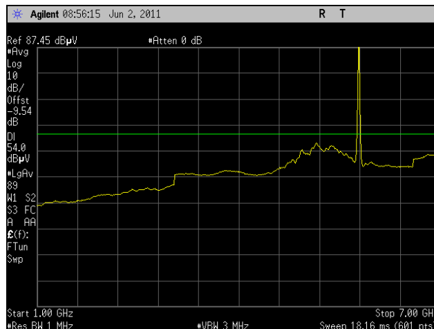
Plot 82. Radiated Spurious Emissions, 802.11a, Mid Channel, 1 GHz – 7 GHz, Average
