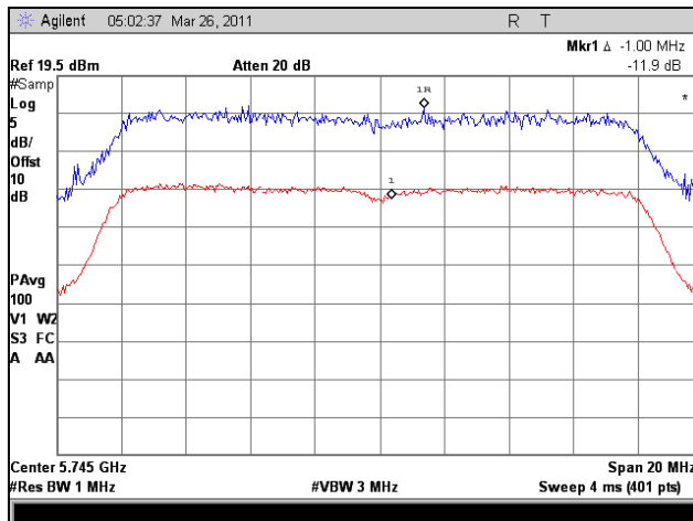
Plot 61. Peak Excursion, 802.11a, Low Channel
