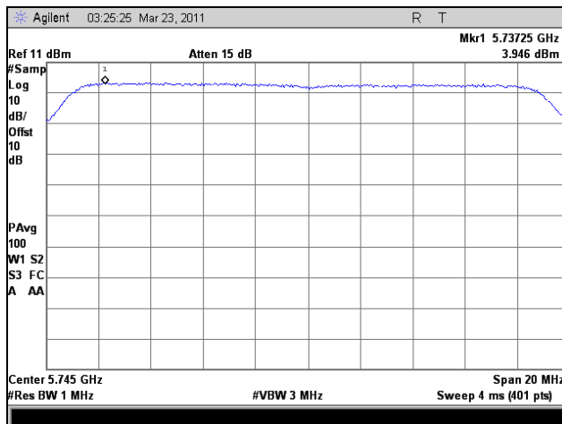
Plot 54. PPSD, 802.11n 20 MHz, Port 1, Low Channel
