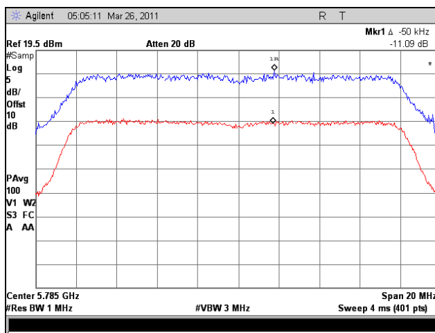
Plot 62. Peak Excursion, 802.11a, Mid Channel
