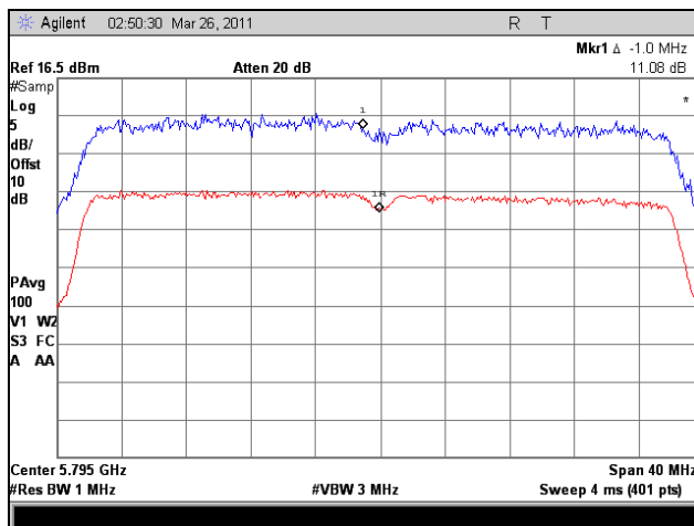
Plot 73. Peak Excursion, 802.11n 40 MHz, Port 1, High Channel
