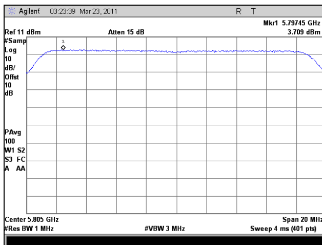
Plot 56. PPSD, 802.11n 20 MHz, Port 1, High Channel
