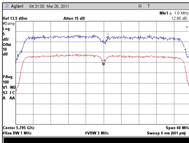
Plot 71. Peak Excursion, 802.11n 40 MHz, Port 0, High Channel
