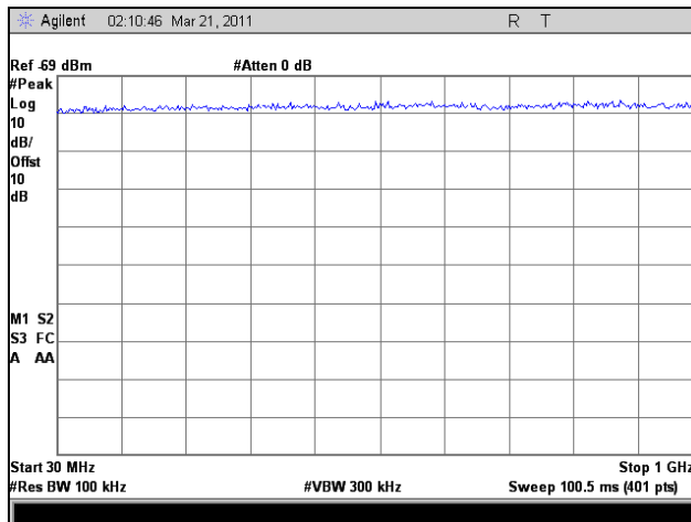
Plot 156. Receiver Spurious Emissions, Port 1, 30 MHz – 1 GHz
