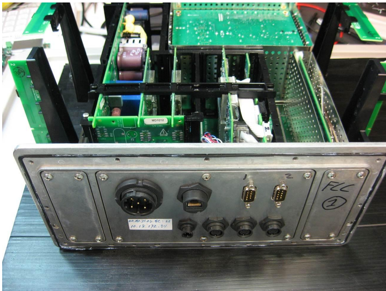
Photograph 10. ECN-70101_Partly Disassembled5-IMG_0285
