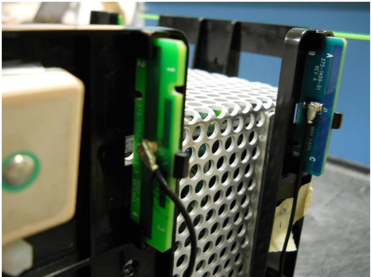
Photograph 14. Left Wi-Fi Antennas from Right Side-1-DSCN0053
