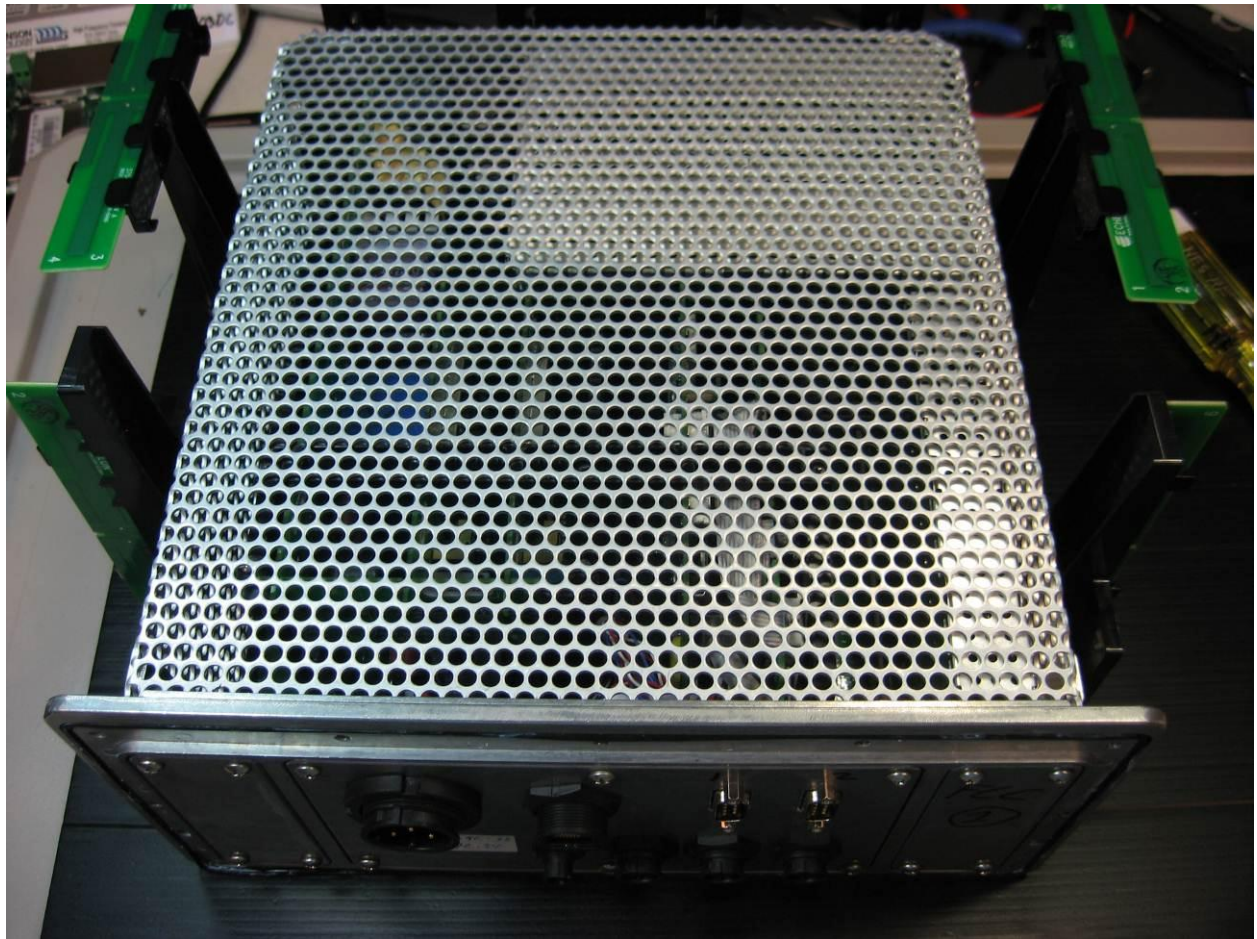
Photograph 7. ECN-70101_Case_Removed1-IMG_0288
