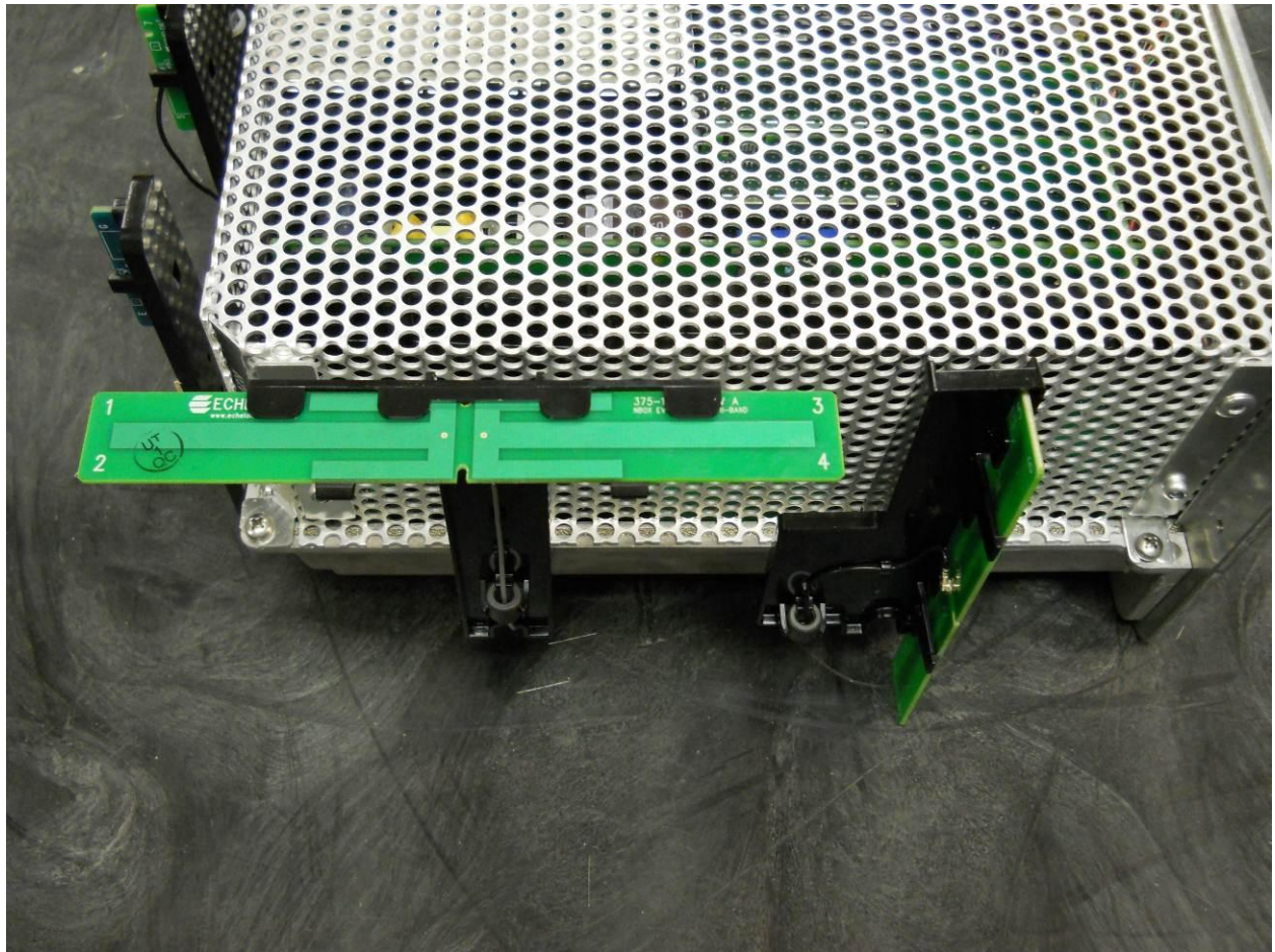
Photograph 17. Primary EV-DO Antenna-DSCN0054
