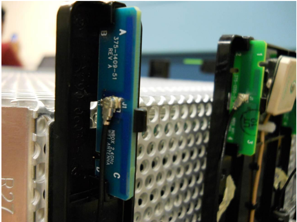
Photograph 19. Right Wi-Fi Antennas from Right Side-1-DSCN0052
