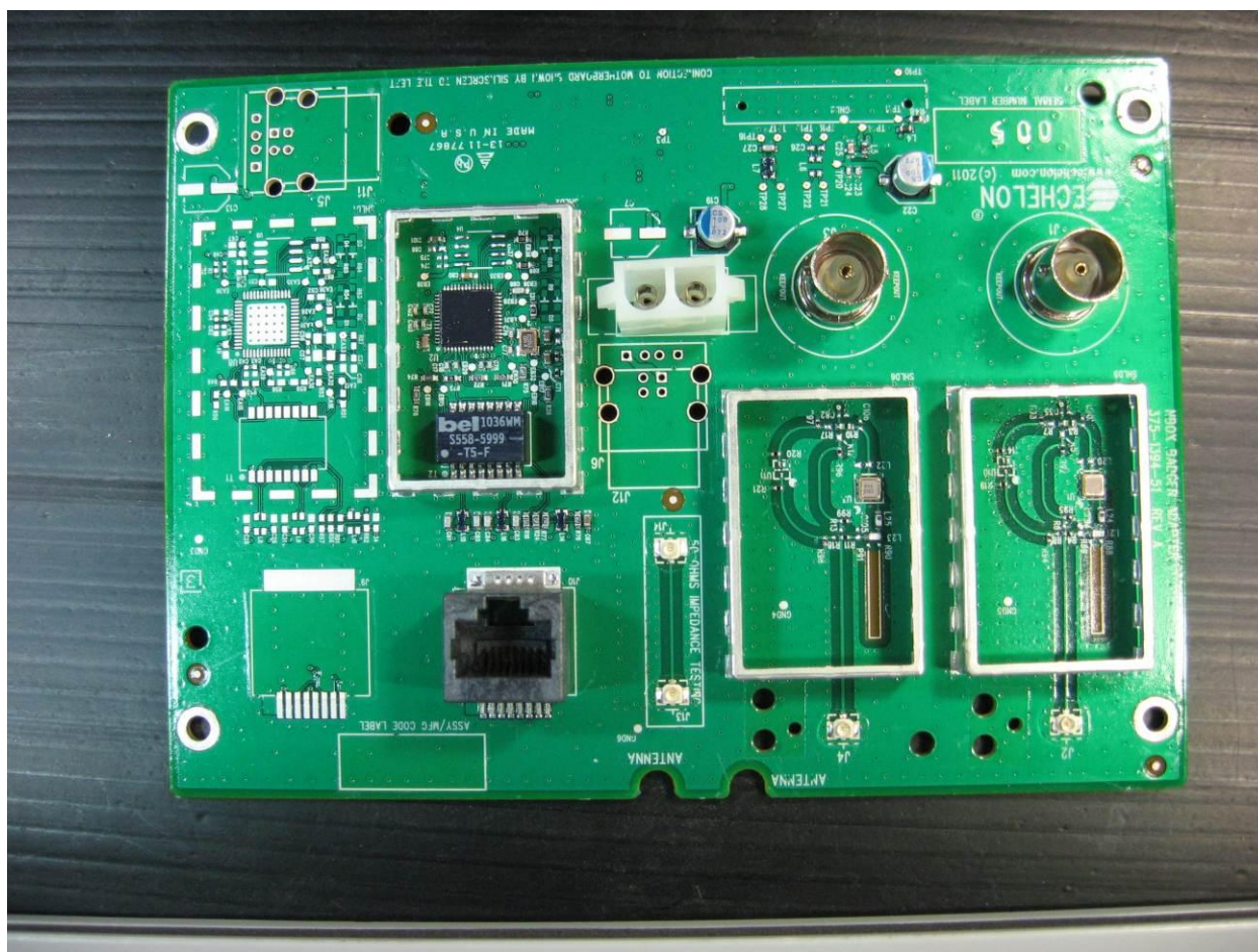
Photograph 2. Badger_IFB_Top1-IMG_0279
