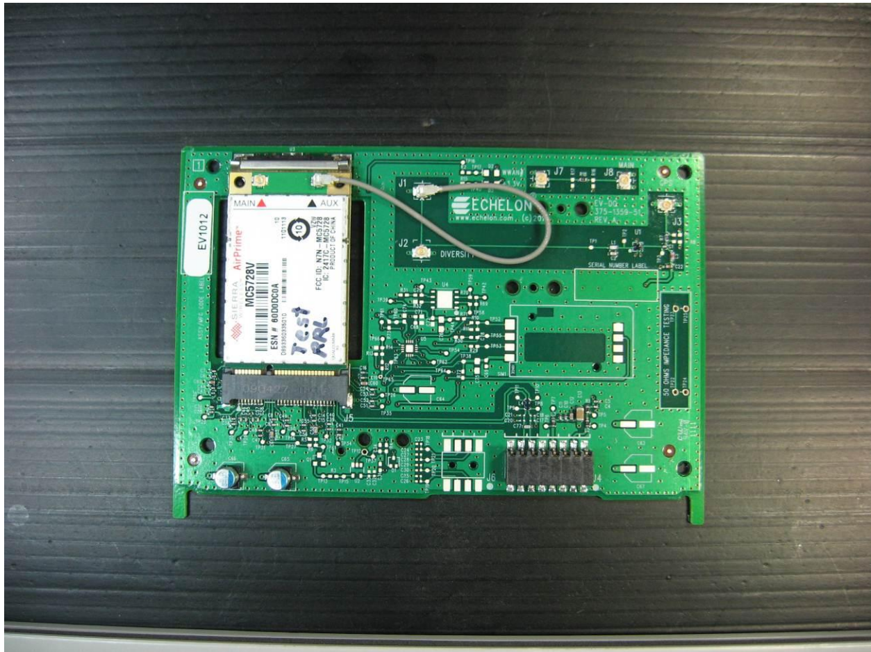
Photograph 13. EV-DO Board_Top1-IMG_0271
