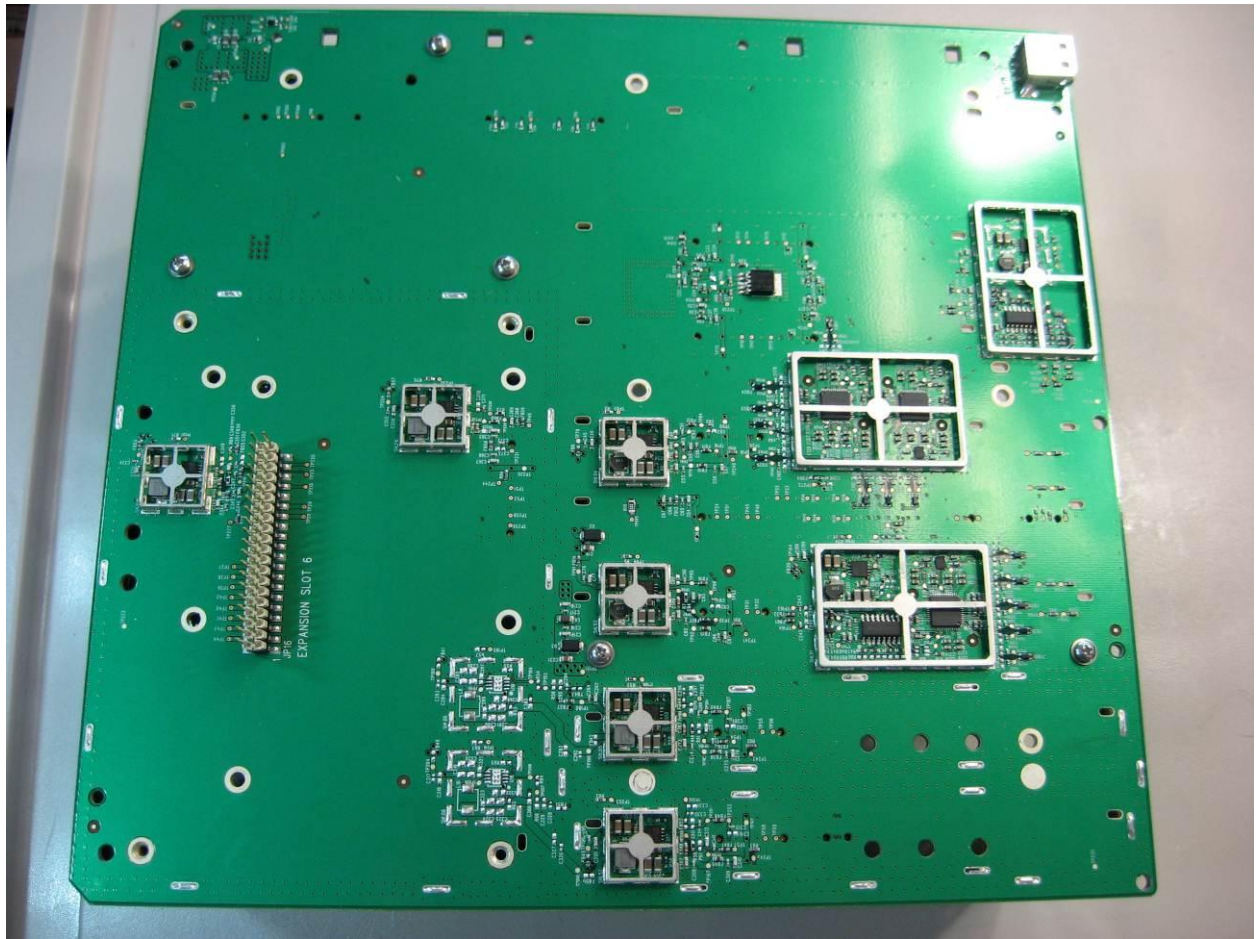
Photograph 23. 375-1354_Motherboard_bottom_I0379
