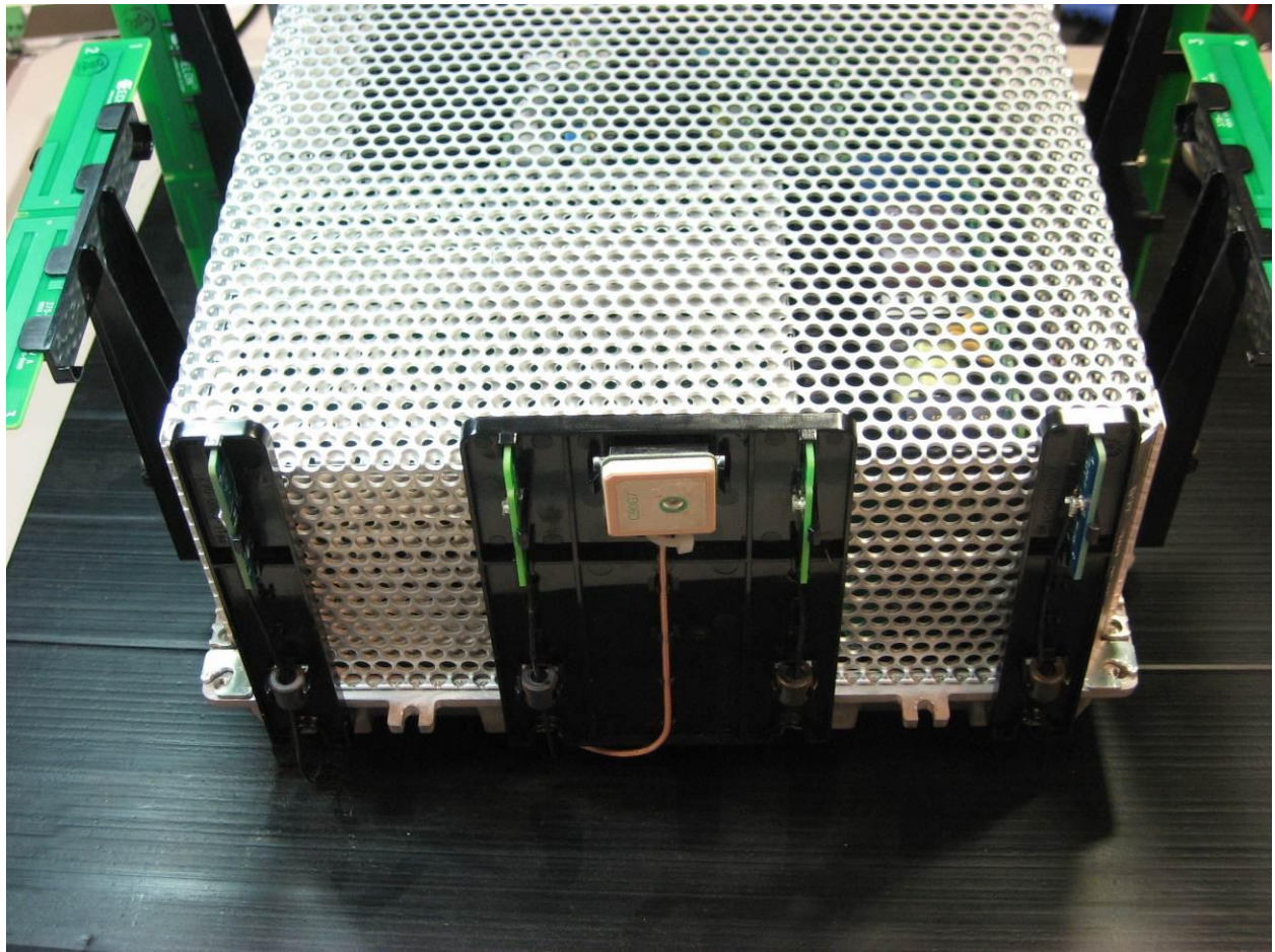
Photograph 8. ECN-70101_Case_Removed2-IMG_0289
