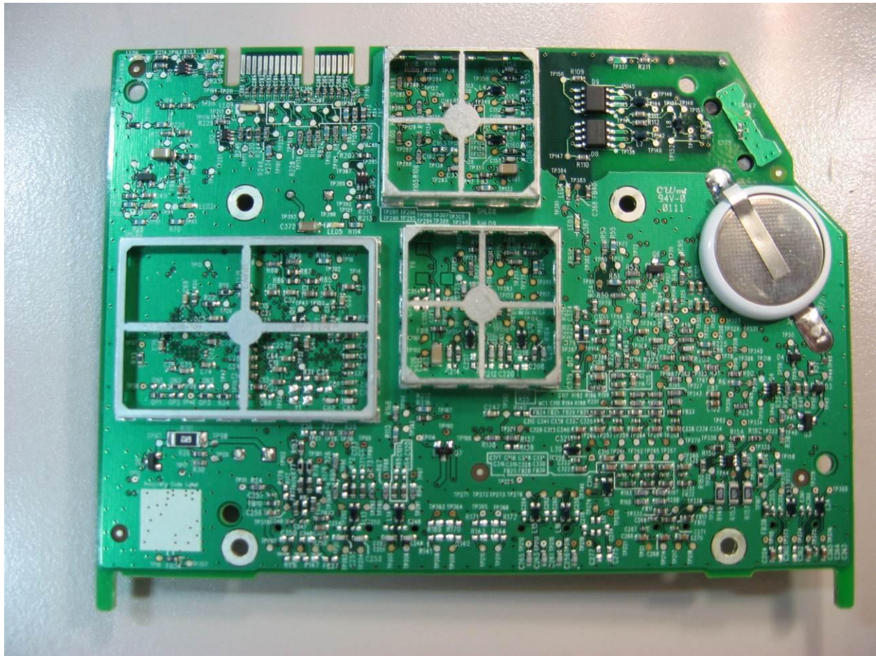
Photograph 21. 375-1353_CPU_Bottom_IO347
