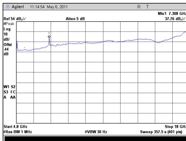
Plot 147. Radiated Spurious Emissions, Mid Channel, 802.11n 20 MHz, 4.8 GHz – 18 GHz, Average, 2.4 GHz
