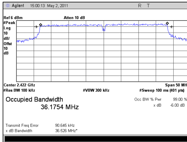
Plot 25. 6 dB Occupied Bandwidth, Low Channel, 802.11n 40 MHz, Port 1, 2.4 GHz
