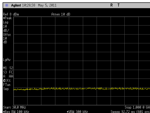
Plot 280. Conducted Spurious Emissions, Mid Channel, 802.11n 20 MHz, Port 1, 30 MHz – 1 GHz, 5.8 GHz
