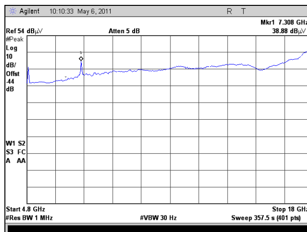
Plot 132. Radiated Spurious Emissions, Mid Channel, 802.11g, 4.8 GHz – 18 GHz, Average, 2.4 GHz
