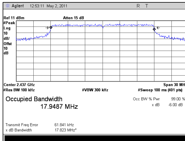
Plot 17. 6 dB Occupied Bandwidth, Mid Channel, 802.11n 20 MHz, Port 0, 2.4 GHz
