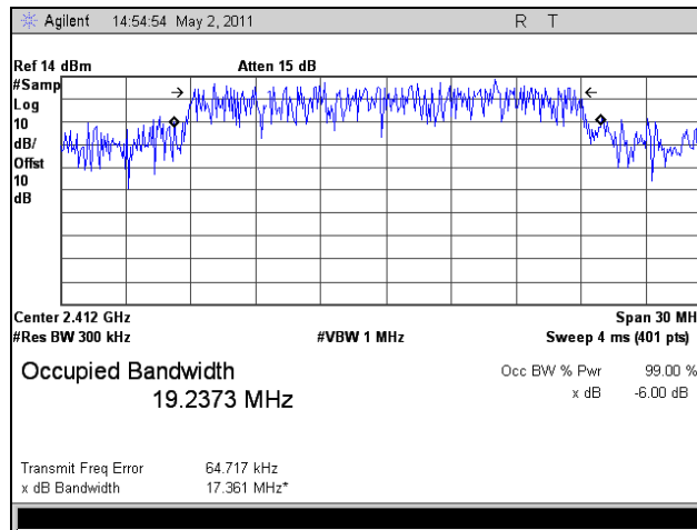
Plot 37. 99% Occupied Bandwidth, Low Channel, 802.11n 20 MHz, Port 1, 2.4 GHz
