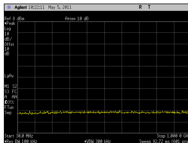
Plot 268. Conducted Spurious Emissions, Mid Channel, 802.11a, 30 MHz – 1 GHz, 5.8 GHz
