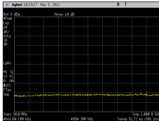
Plot 278. Conducted Spurious Emissions, Low Channel, 802.11n 20 MHz, Port 1, 30 MHz – 1 GHz, 5.8 GHz
