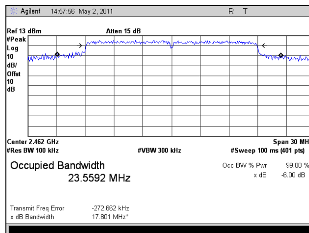
Plot 21. 6 dB Occupied Bandwidth, High Channel, 802.11n 20 MHz, Port 1, 2.4 GHz
