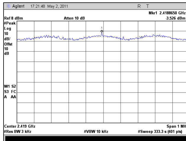
Plot 327. Peak Power Spectral Density, Low Channel, 802.11n 40 MHz, Port 1, 2.4 GHz
