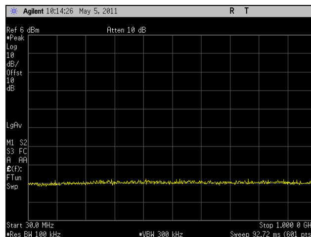
Plot 292. Conducted Spurious Emissions, Mid Channel, 802.11n 40 MHz, Port 1, 30 MHz – 1 GHz, 5.8 GHz
