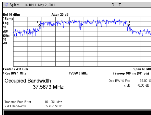
Plot 41. 99% Occupied Bandwidth, Mid Channel, 802.11n 40 MHz, Port 0, 2.4 GHz
