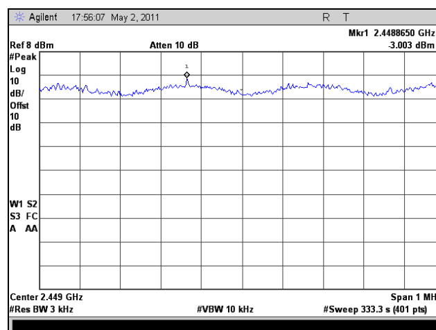
Plot 329. Peak Power Spectral Density, High Channel, 802.11n 40 MHz, Port 1, 2.4 GHz
