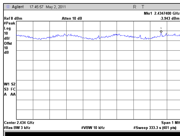
Plot 328. Peak Power Spectral Density, Mid Channel, 802.11n 40 MHz, Port 1, 2.4 GHz
