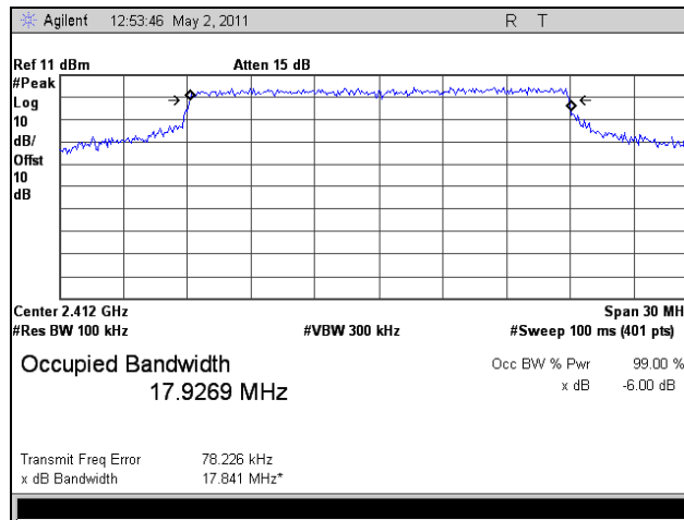
Plot 16. 6 dB Occupied Bandwidth, Low Channel, 802.11n 20 MHz, Port 0, 2.4 GHz
