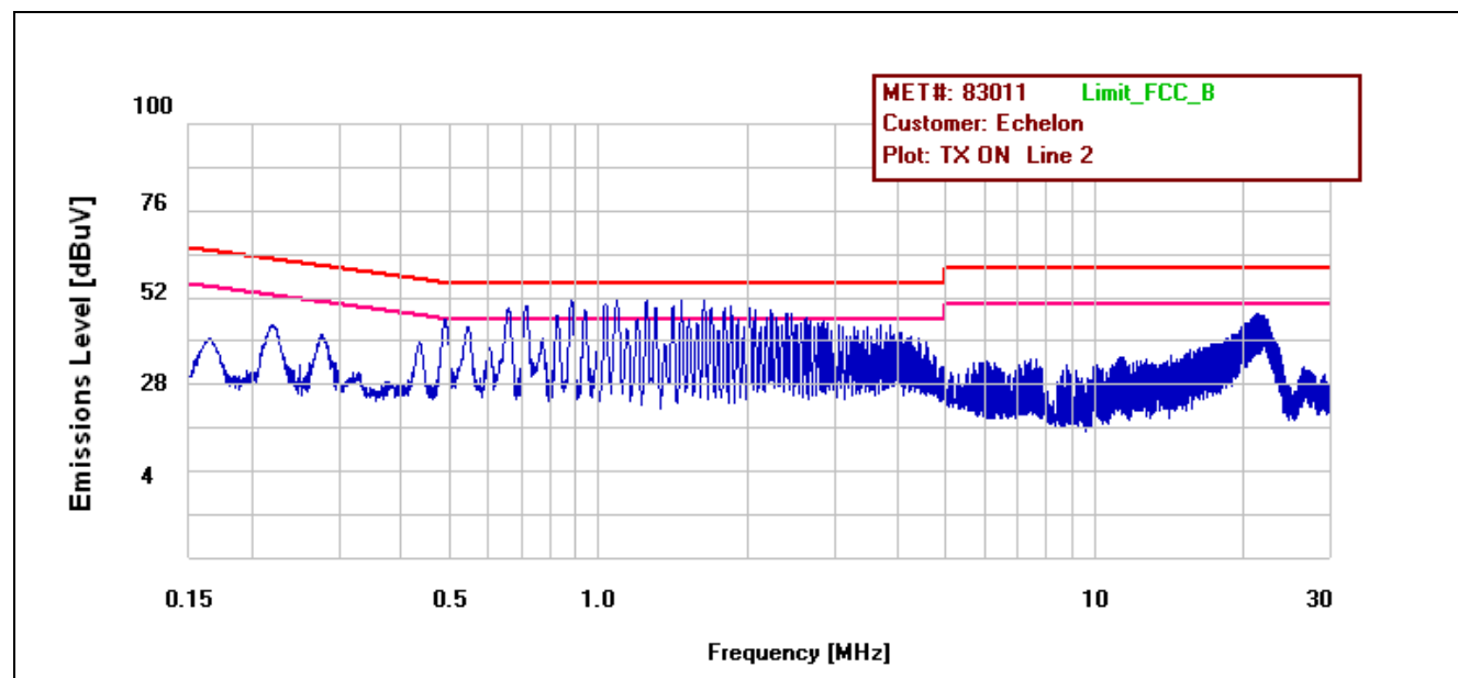
Plot 8. Conducted Emissions, 15.207(a), TX ON, Line 2
