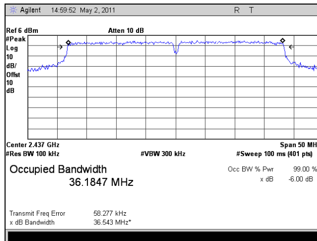
Plot 26. 6 dB Occupied Bandwidth, Mid Channel, 802.11n 40 MHz, Port 1, 2.4 GHz
