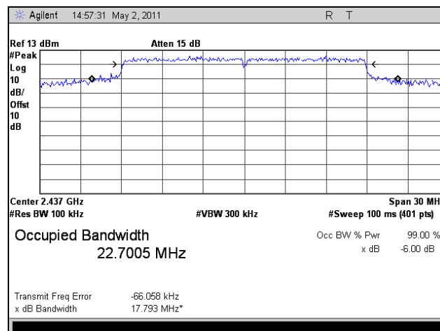
Plot 20. 6 dB Occupied Bandwidth, Mid Channel, 802.11n 20 MHz, Port 1, 2.4 GHz
