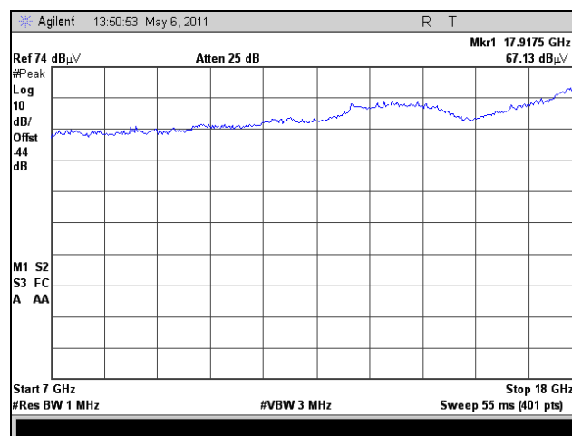
Plot 183. Radiated Spurious Emissions, High Channel, 802.11a, 7 GHz – 18 GHz, Peak, 5.8 GHz
