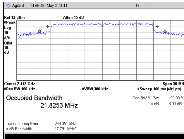
Plot 19. 6 dB Occupied Bandwidth, Low Channel, 802.11n 20 MHz, Port 1, 2.4 GHz
