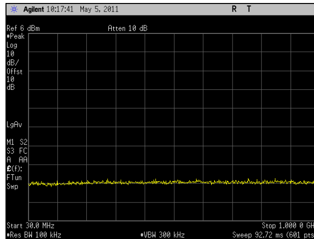
Plot 290. Conducted Spurious Emissions, Low Channel, 802.11n 40 MHz, Port 1, 30 MHz – 1 GHz, 5.8 GHz
