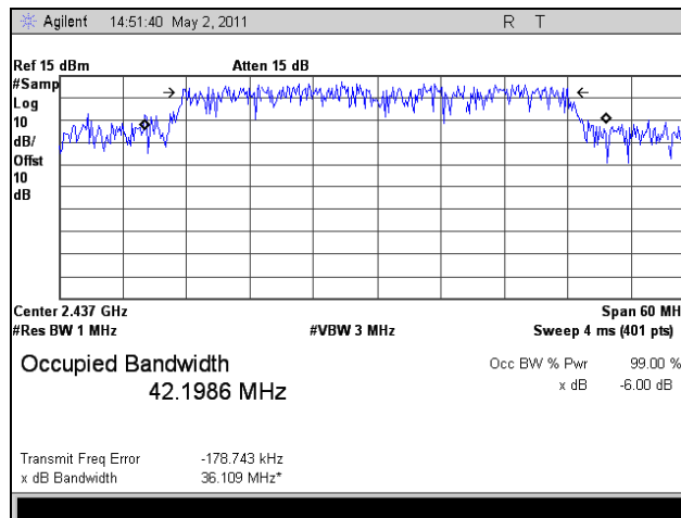
Plot 44. 99% Occupied Bandwidth, Mid Channel, 802.11n 40 MHz, Port 1, 2.4 GHz
