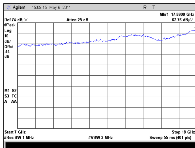
Plot 213. Radiated Spurious Emissions, High Channel, 802.11n 40 MHz, 7 GHz – 18 GHz, Peak, 5.8 GHz
