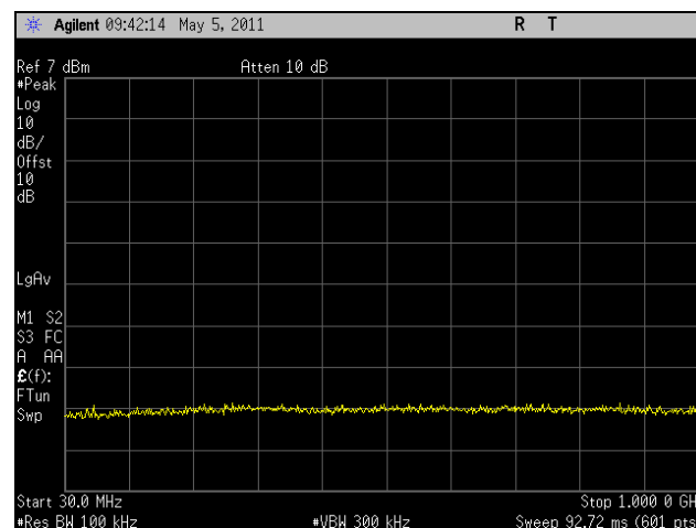
Plot 274. Conducted Spurious Emissions, Mid Channel, 802.11n 20 MHz, Port 0, 30 MHz – 1 GHz, 5.8 GHz
