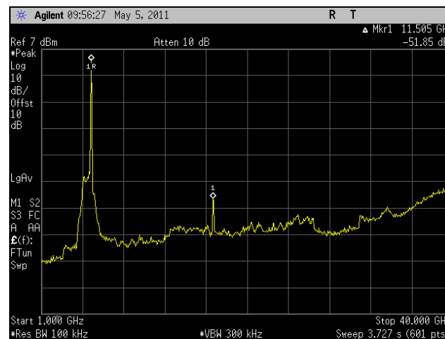
Plot 285. Conducted Spurious Emissions, Low Channel, 802.11n 40 MHz, Port 0, 1 GHz – 40 GHz, 5.8 GHz
