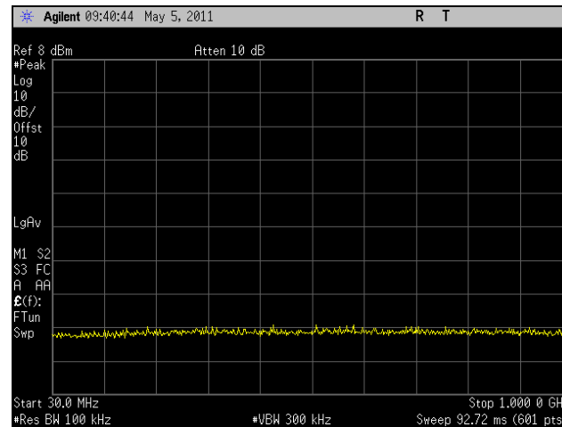
Plot 272. Conducted Spurious Emissions, Low Channel, 802.11n 20 MHz, Port 0, 30 MHz – 1 GHz, 5.8 GHz
