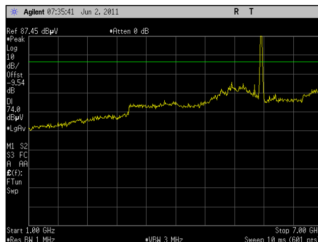
Plot 171. Radiated Spurious Emissions, Low Channel, 802.11a, 1 GHz – 7 GHz, Peak, 5.8 GHz
