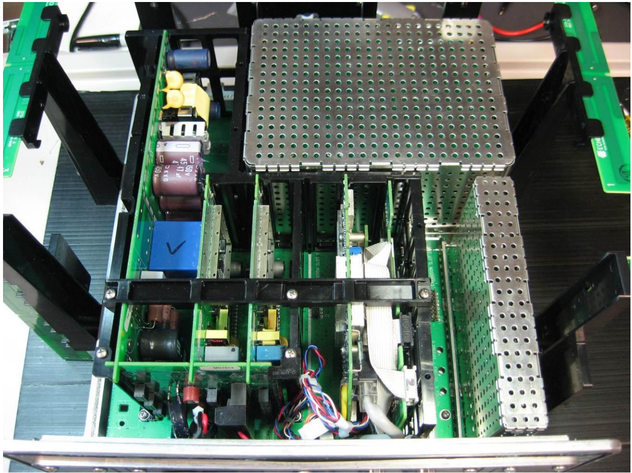
Photograph 14. ECN-70101_Partly Disassembled6-IMG_0286
