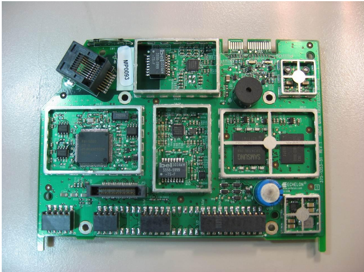
Photograph 17. 375-1353_CPU_I0345
