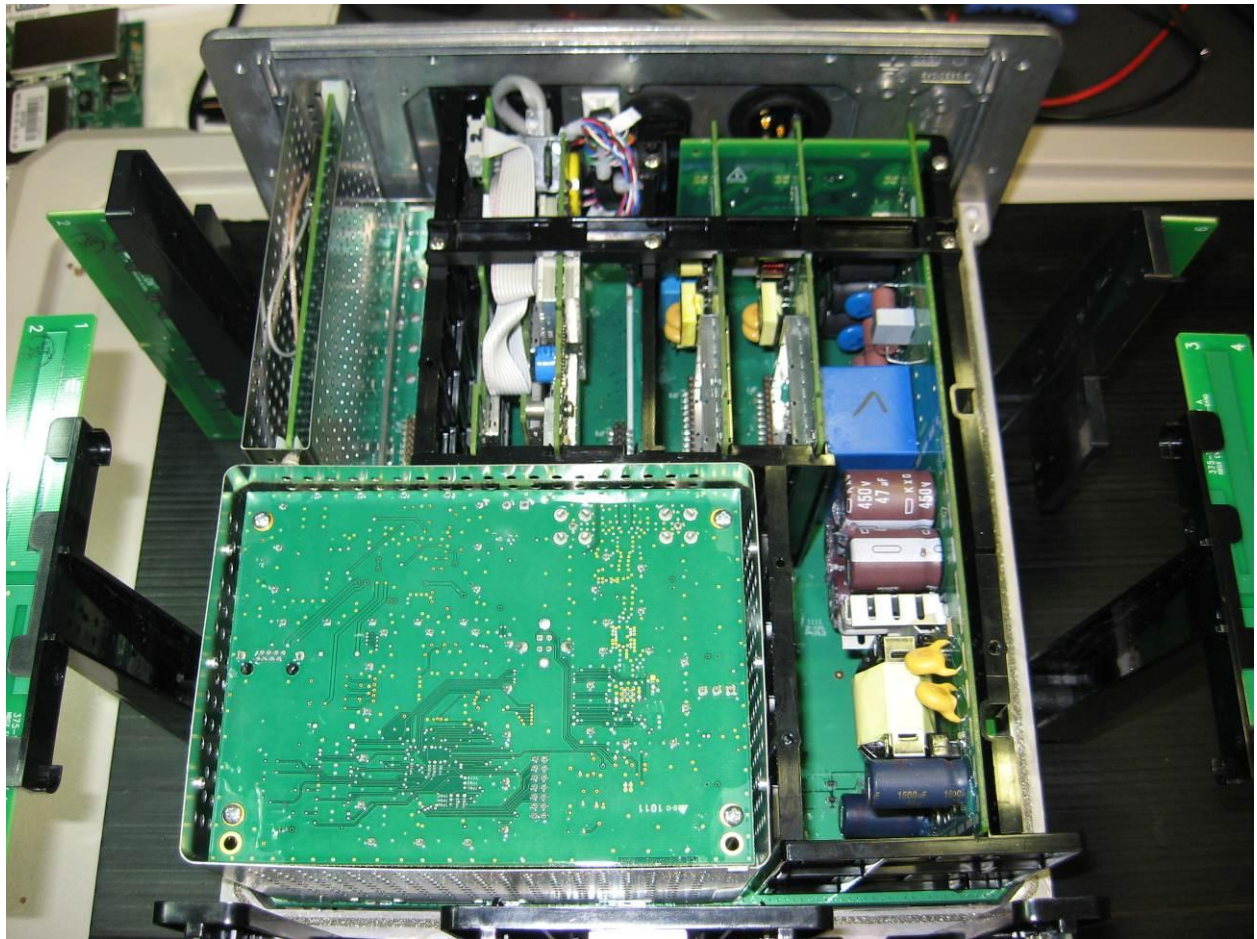
Photograph 12. ECN-70101_Partly Disassembled3-IMG_0283
