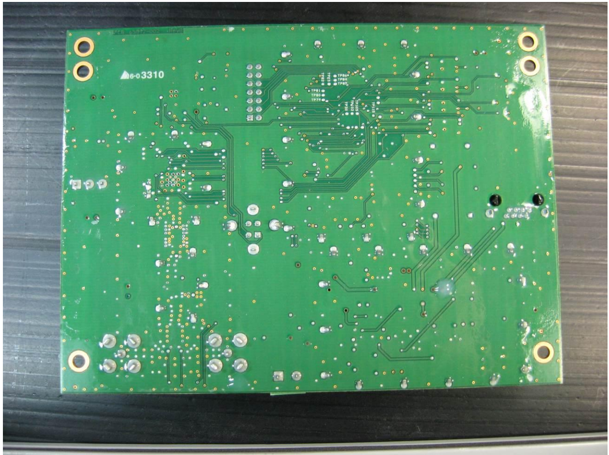
Photograph 8. Badger_Orion-GW_Bottom1-IMG_0278
