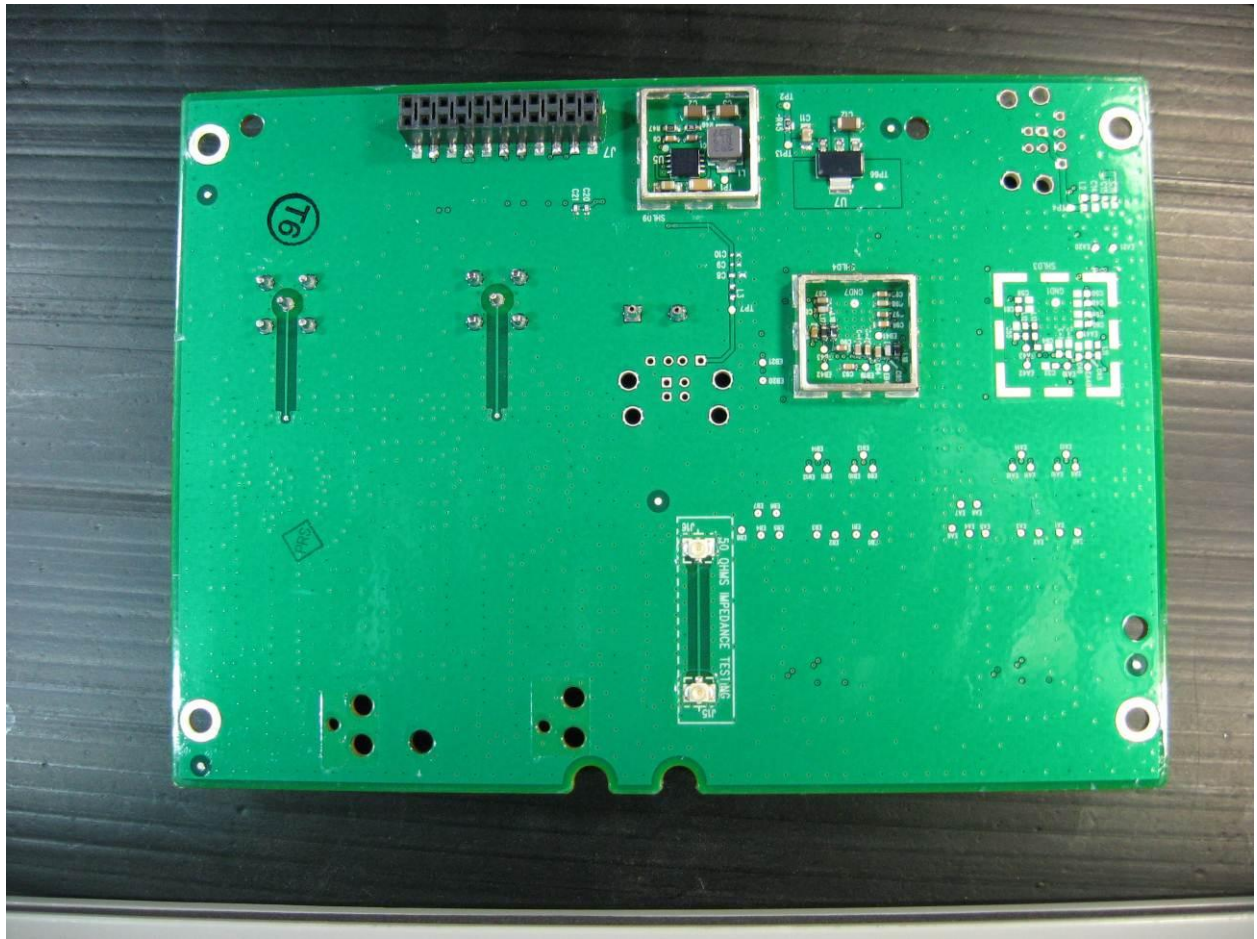
Photograph 6. Badger_IFB_Bottom1-IMG_0280
