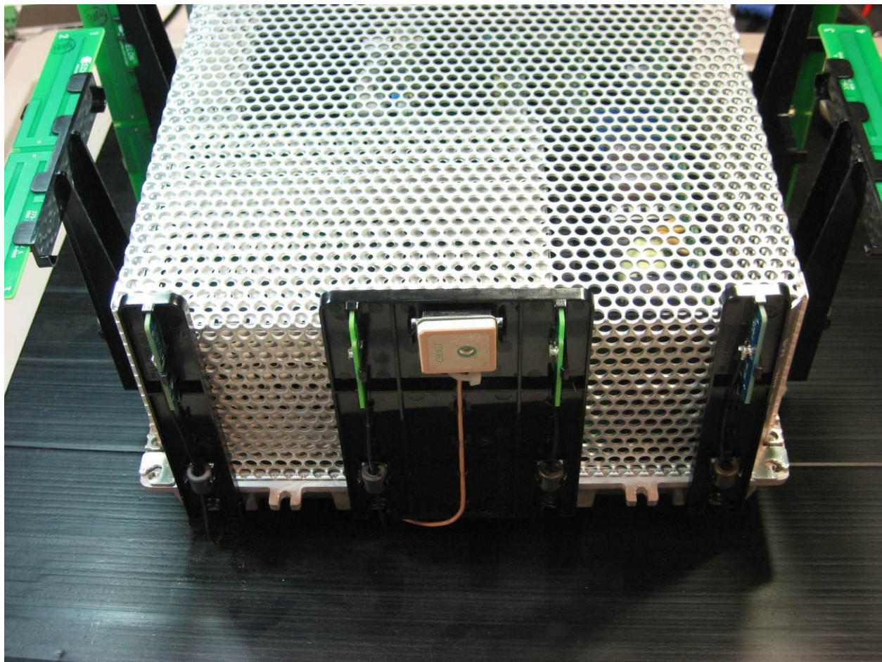
Photograph 11. ECN-70101_Case_Removed2-IMG_0289
