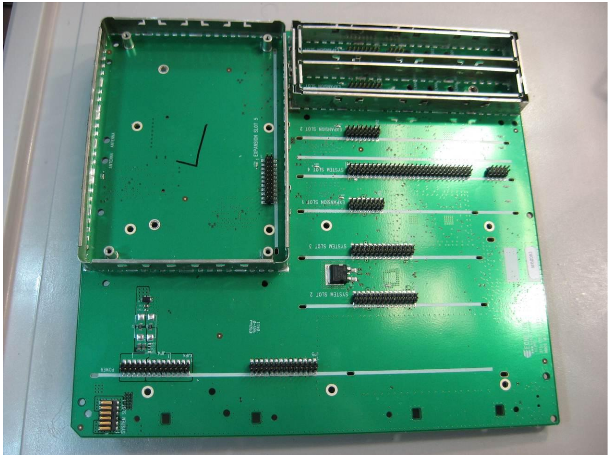
Photograph 19. 375-1354_Motherboard_I0382
