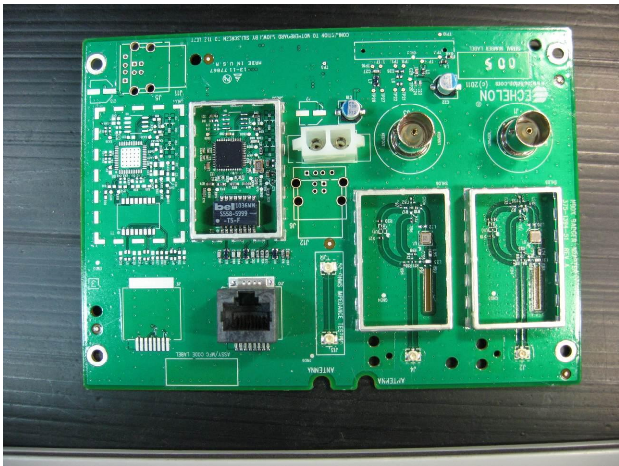
Photograph 7. Badger_IFB_Top1-IMG_0279
