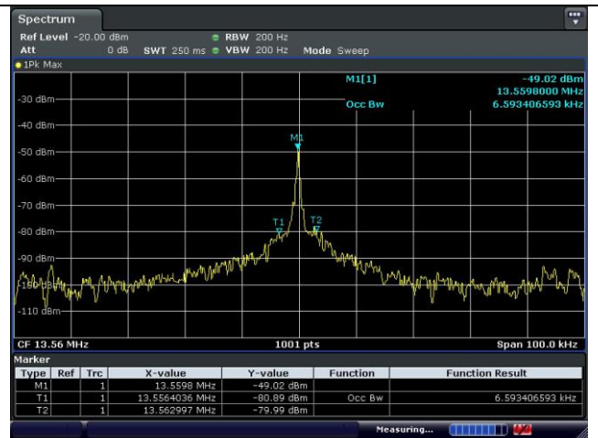
99 % Bandwidth
