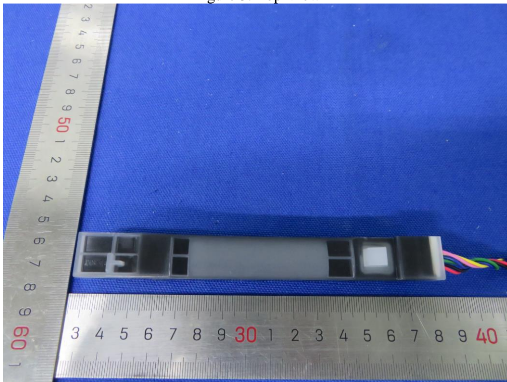
Figure 6. Bottom View
