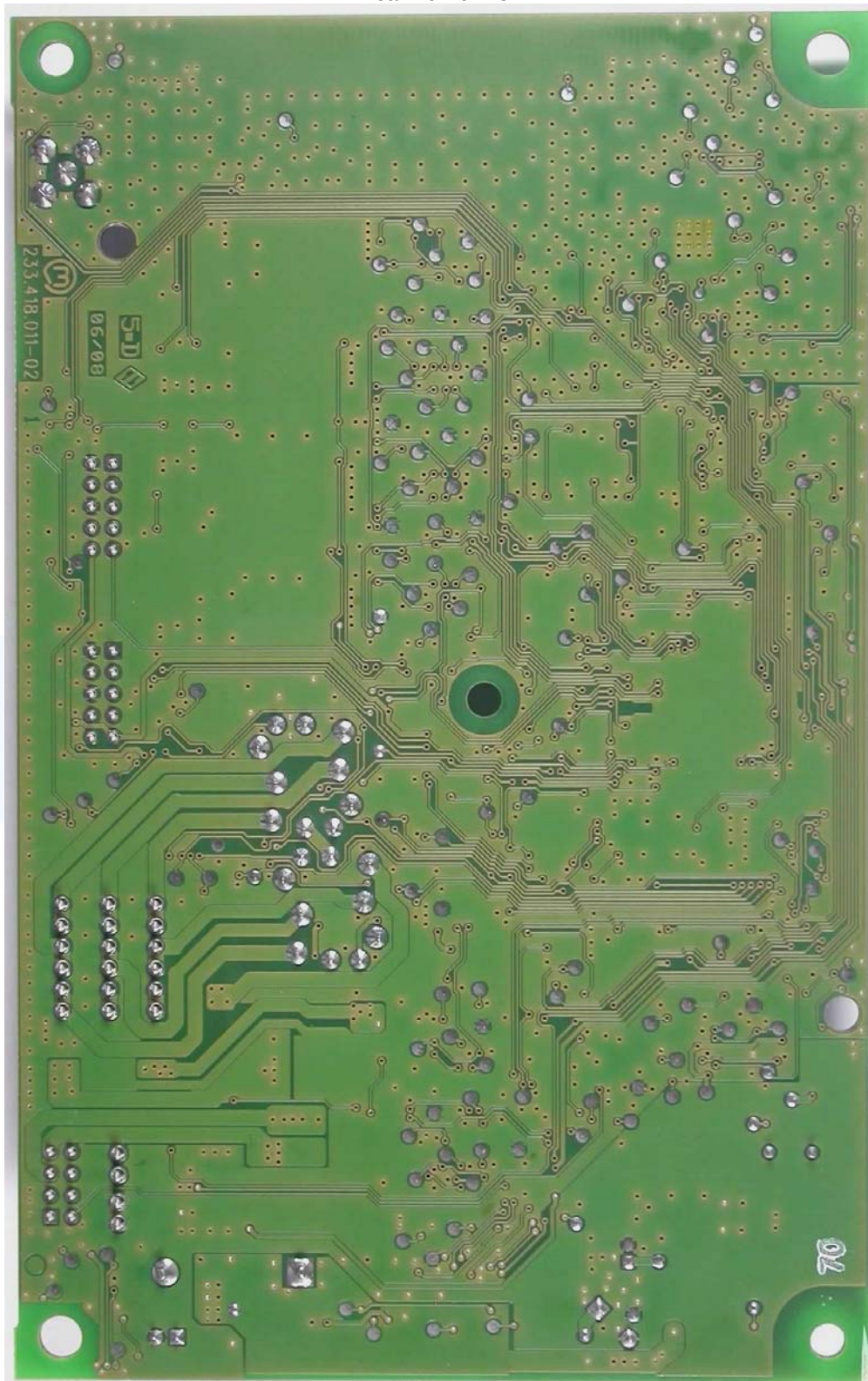
Rear view of PCB
