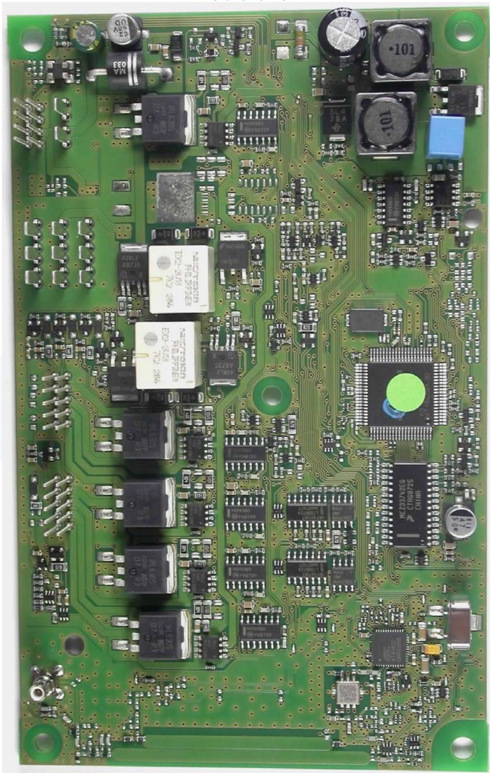
Front view of PCB
