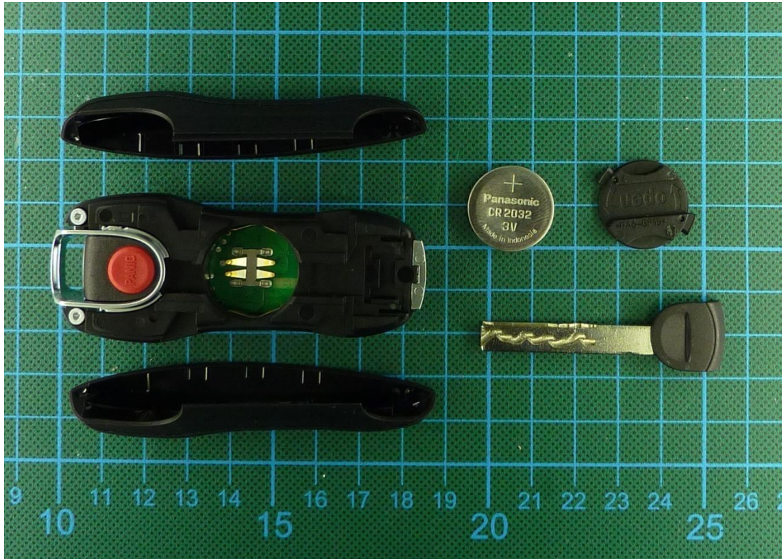
171908_19.JPG: EUT - bottom view - battery cover removed
