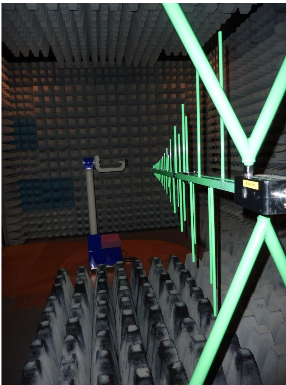
171908_14.JPG: Test setup fully anechoic chamber
