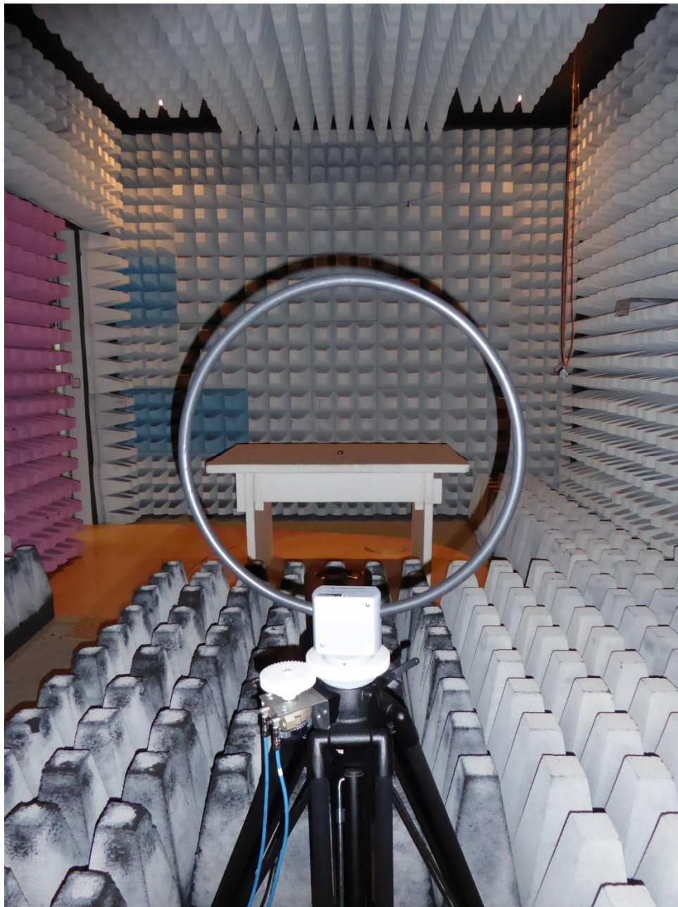
171908_13.JPG: Test setup fully anechoic chamber
