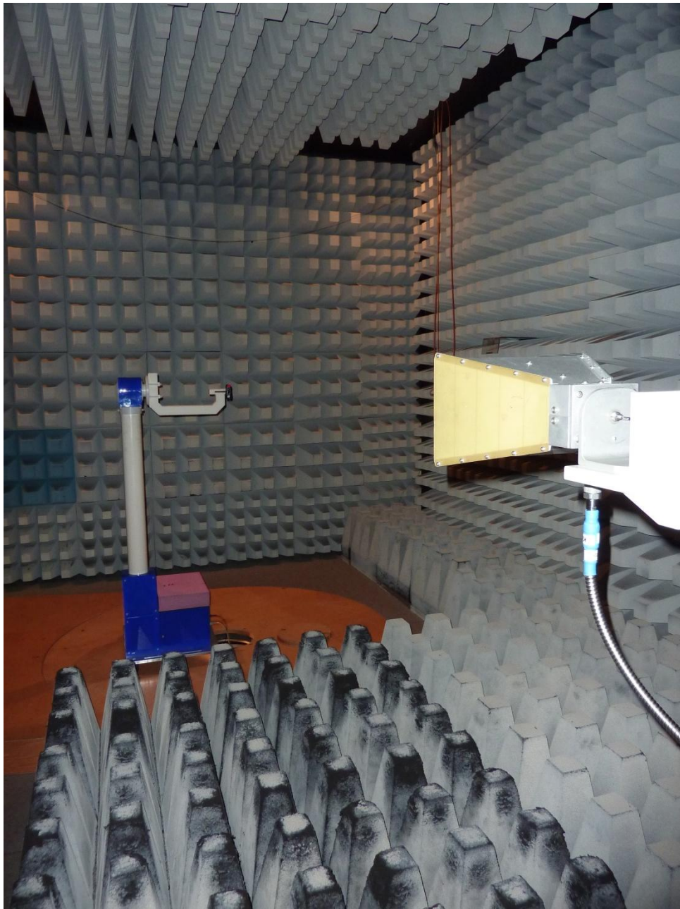
171908_15.JPG: Test setup fully anechoic chamber
