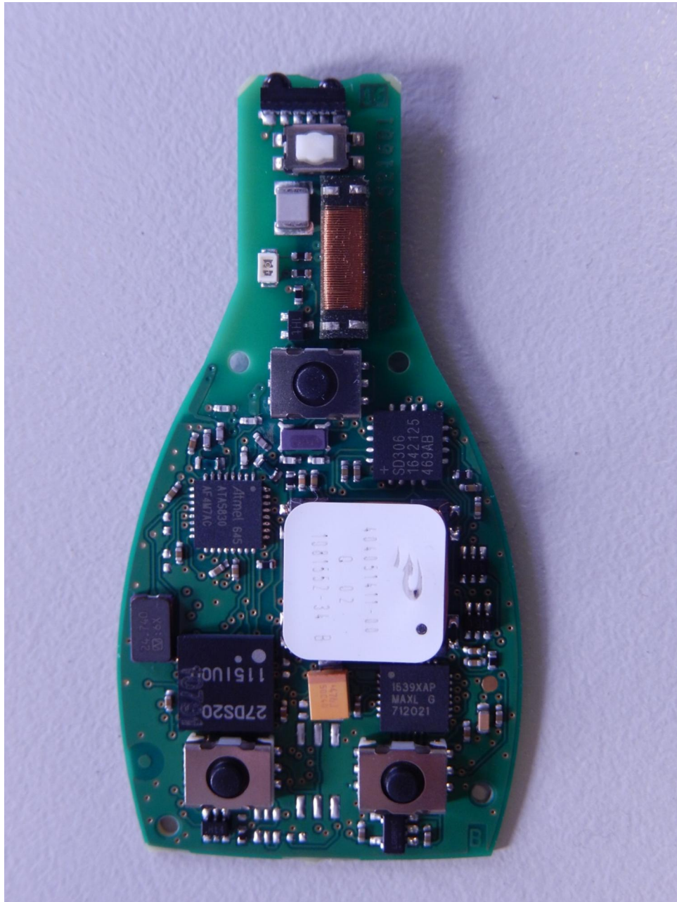
153783_19.JPG: DC12A, PCB, top view
