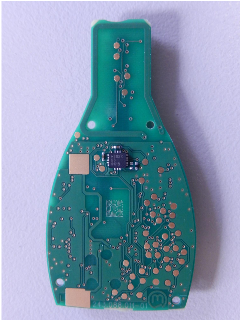
153783_18.JPG: DC12A, PCB, bottom view
