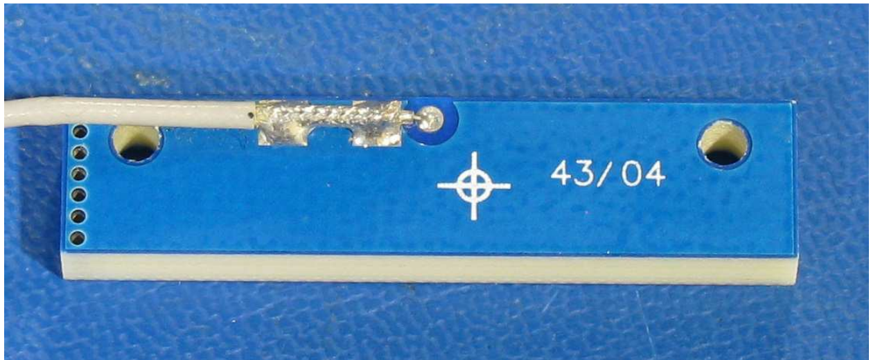
External Antenna Photos
