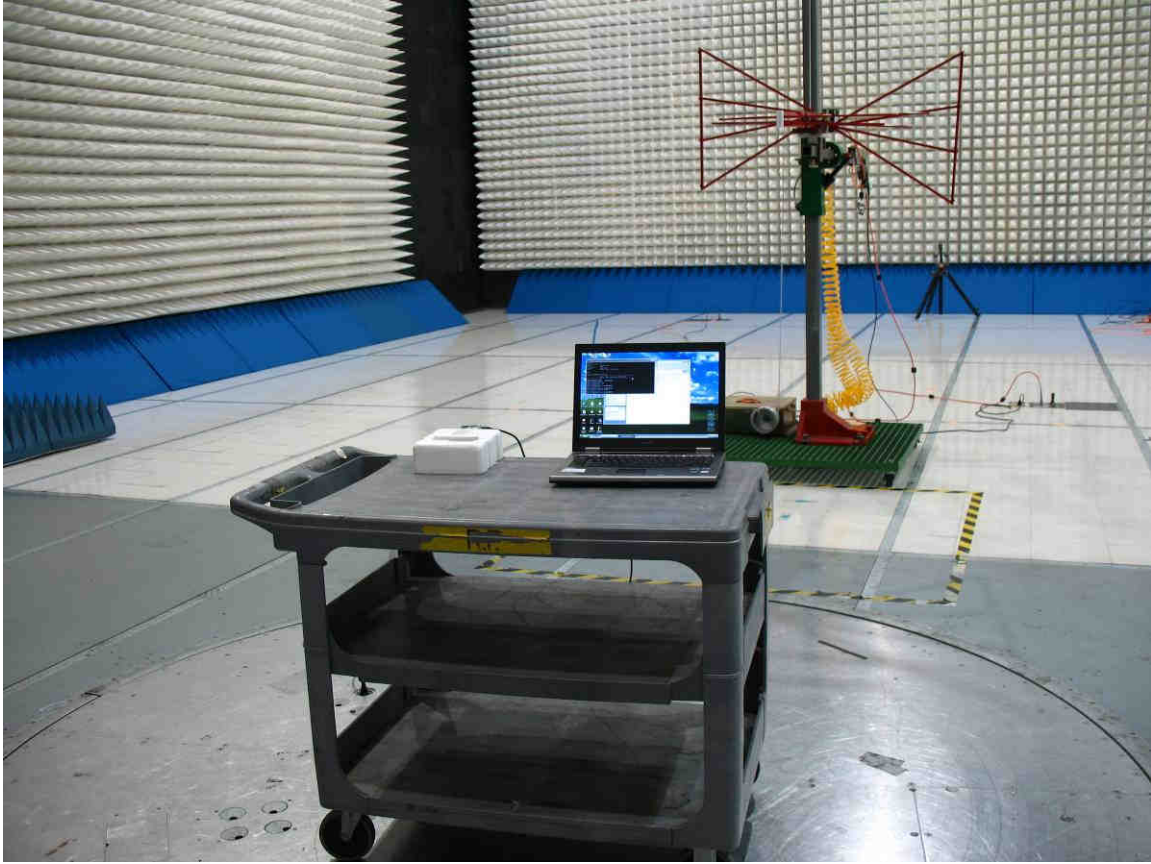
Radiated Emissions
