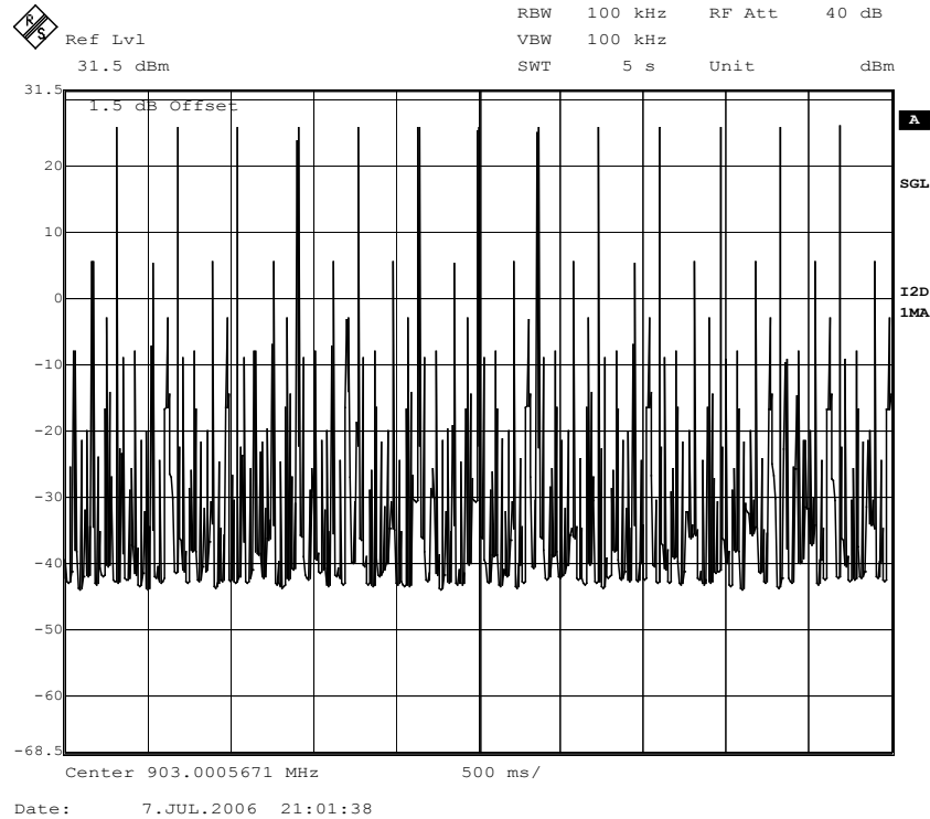
Figure 21. Number of ON events in a 5 second sweep; Channel 1.
