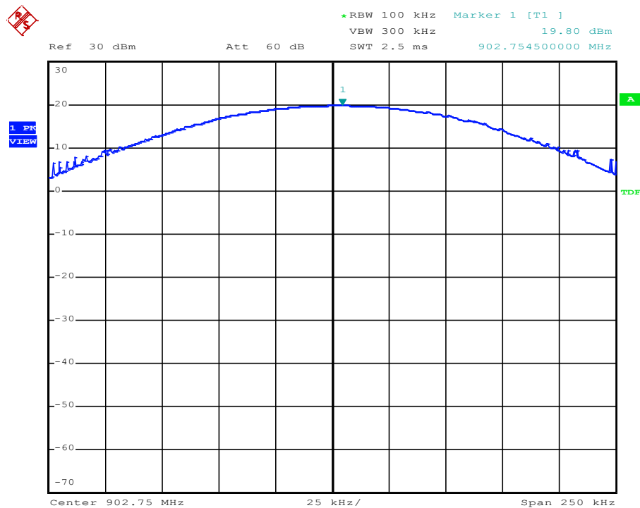
Figure 16. Conducted output power, Channel 1, highest power setting. Voltage = 20.4 VDC.
