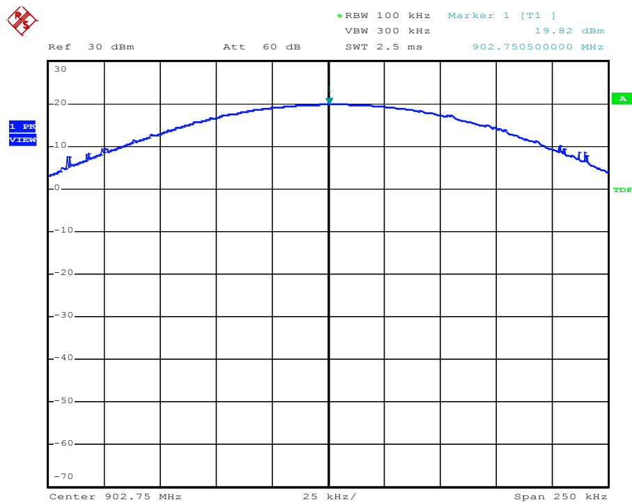
Figure 15. Conducted output power, Channel 1, highest power setting. Voltage = 24 VDC.
