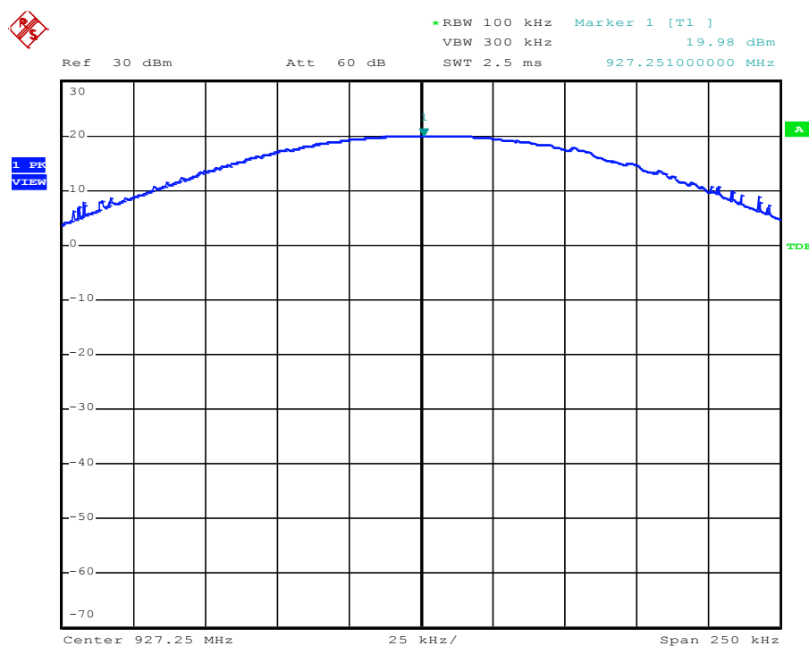
Figure 23. Conducted output power, Channel 50, highest power setting. Voltage = 27.6 VDC.
