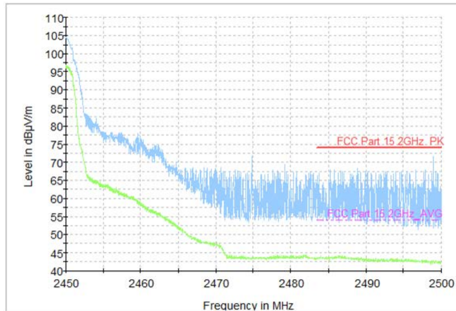
Fig.77 Radiated Restricted Band (802.11n HT40, CH11, 2.45GHz~2.5GHz)
