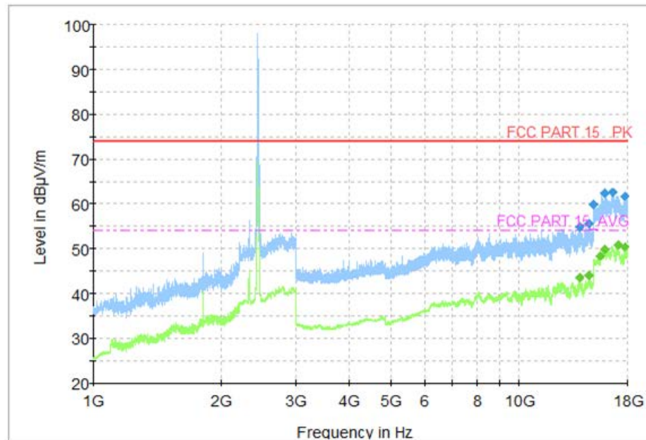
Fig.51 Radiated Spurious Emission (802.11g, CH6, 1 GHz-18 GHz)
