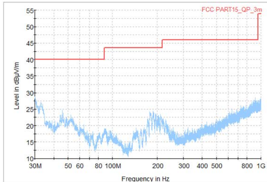
Fig.79 Radiated Spurious Emission (All Channels, 30MHz-1 GHz)
