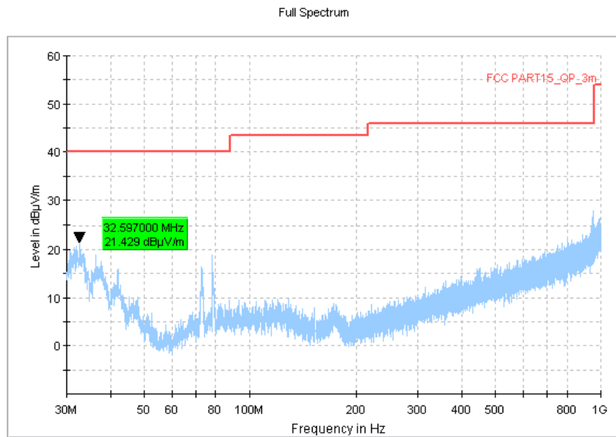
Fig.26 Radiated Spurious Emission (All Channels, 30 MHz-1 GHz)
