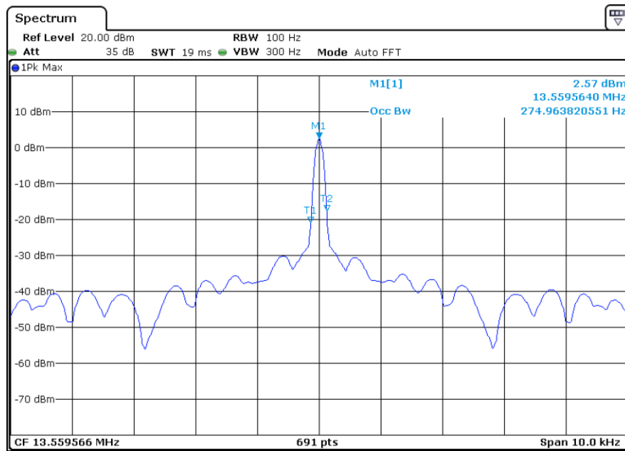
Figure A-6 Occupied Bandwidth
