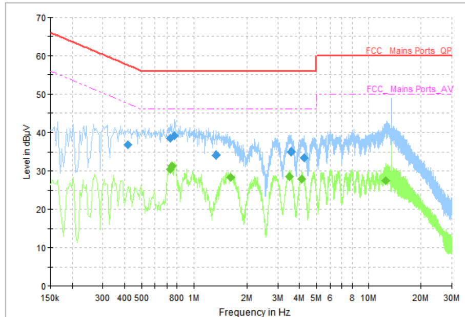
Figure A-5 Test result (120V)
