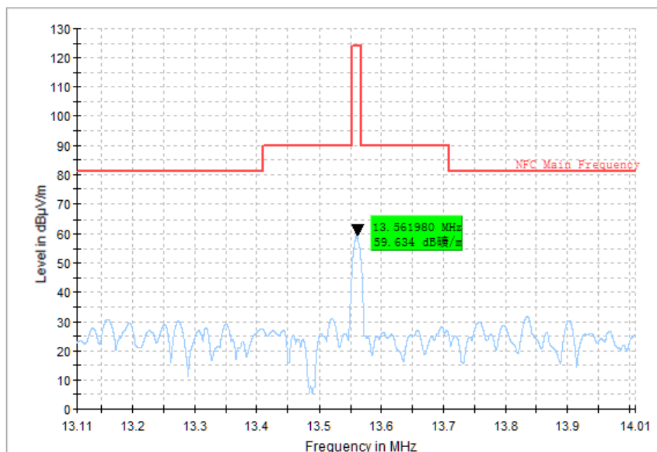
Figure A-1 Electric Field Strength
