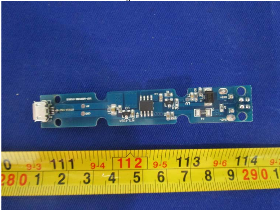
EUT – Charger Mb Bottom View
