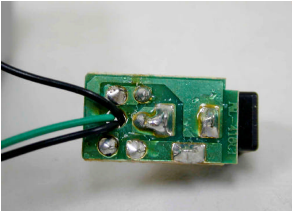
15. Rear view of PCB 5
