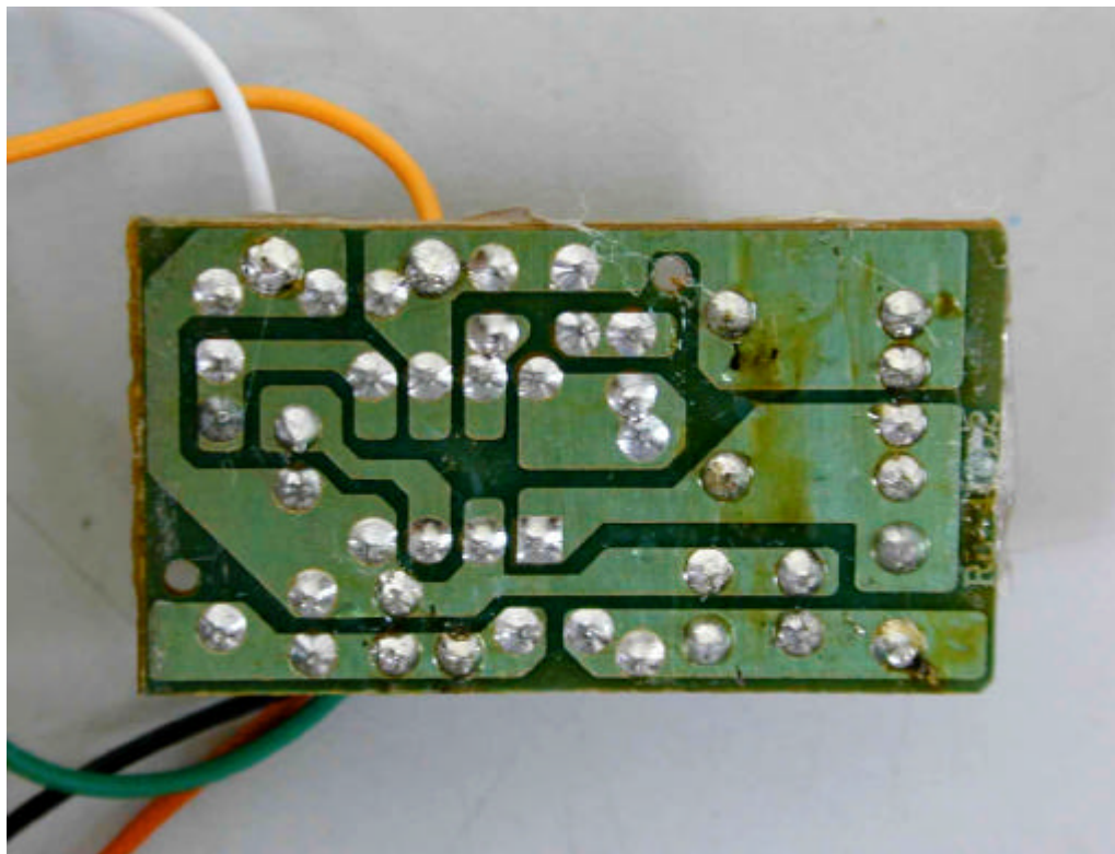
13. Rear view of PCB 4
