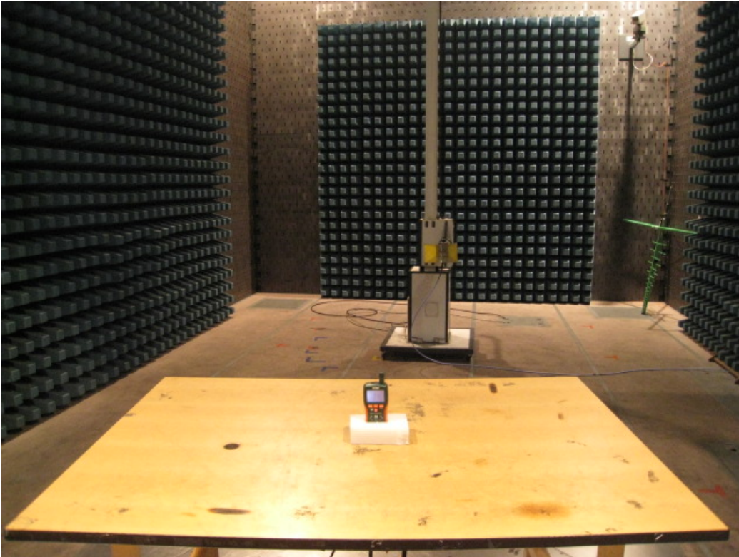
Photo 3 Front of Radiated Disturbance Test (Above 1GHz)
