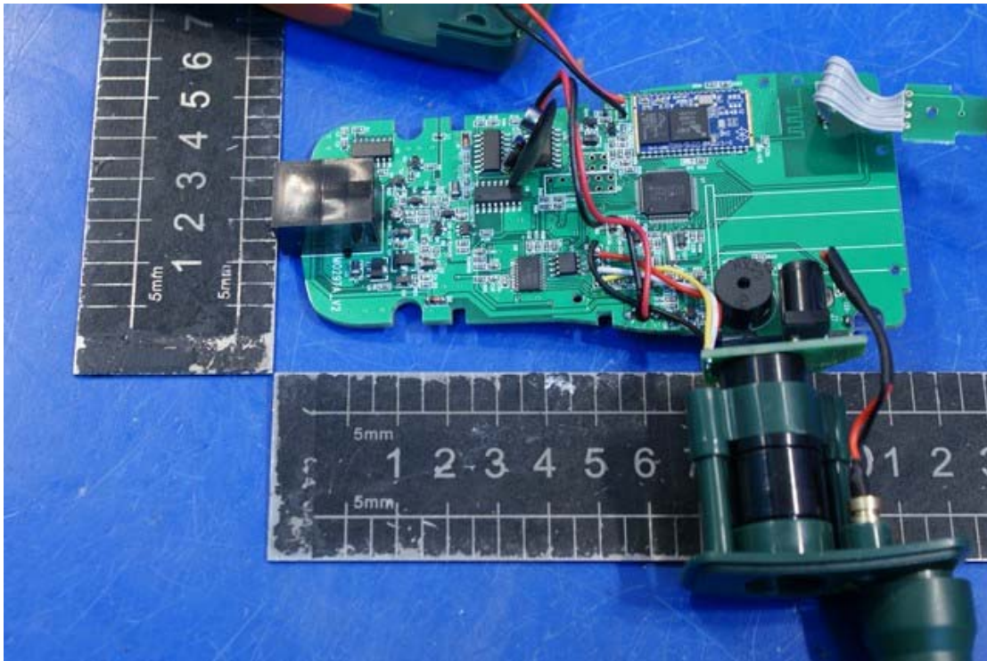
Photo 2 Bluetooth Module (with RF module)
