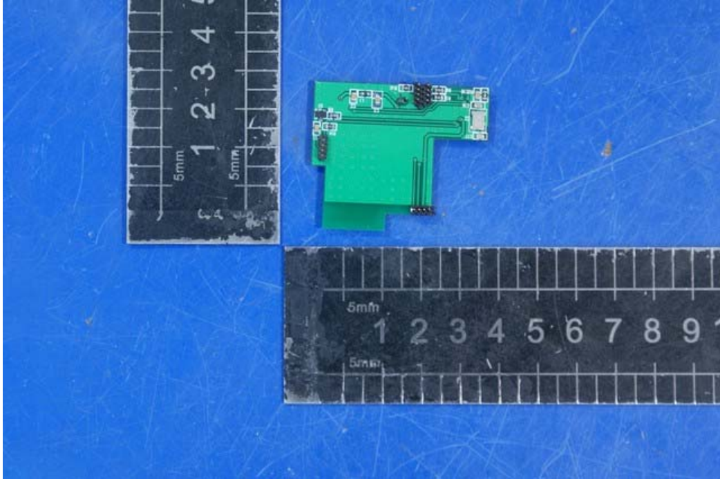
Photo 5 Bluetooth Module (bottom)
