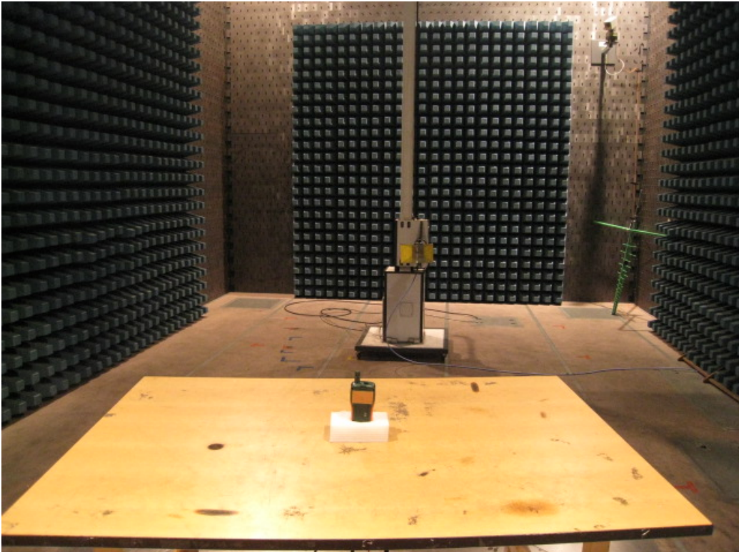
Photo 4 Rear of Radiated Disturbance Test (Above 1GHz)
