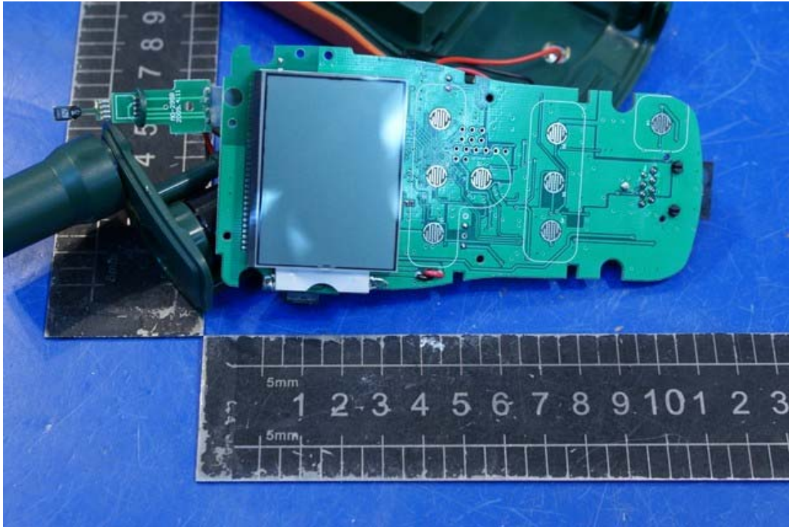
Photo 4 Bluetooth Module (top)
