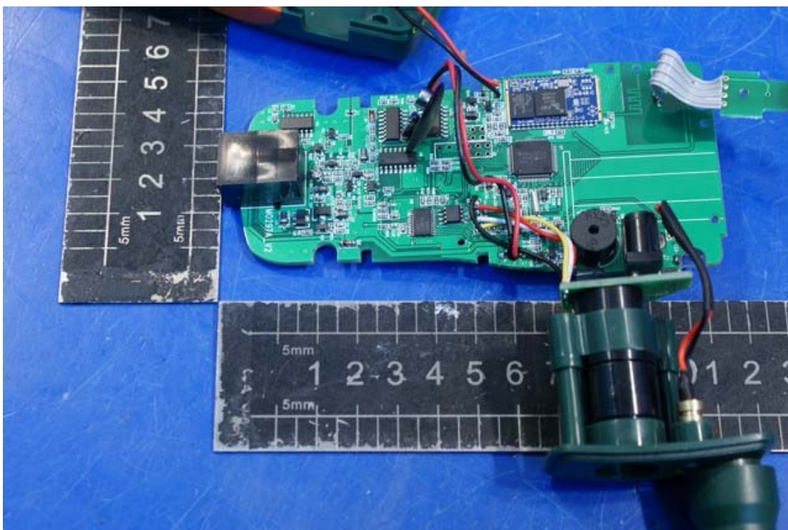
Photo 2 Inside of EUT (with RF module)
