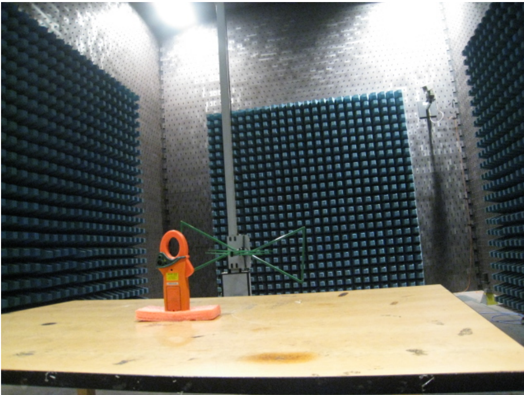
Photo 2 Rear of Radiated Disturbance Test (Below 1GHz)
