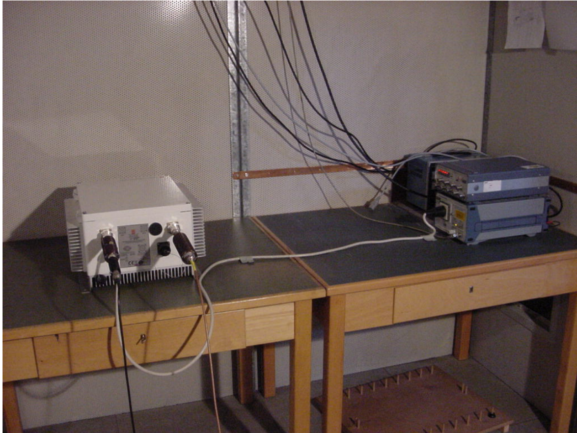
Photo 3: Conducted Emissions
