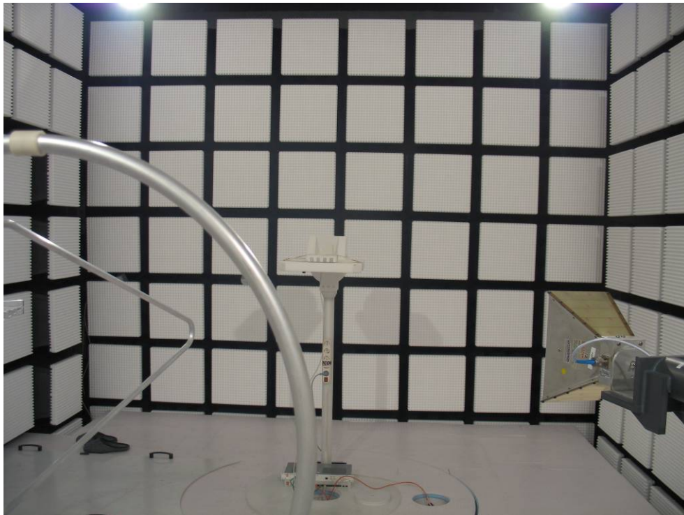
Photo 5: Radiated Emissions
