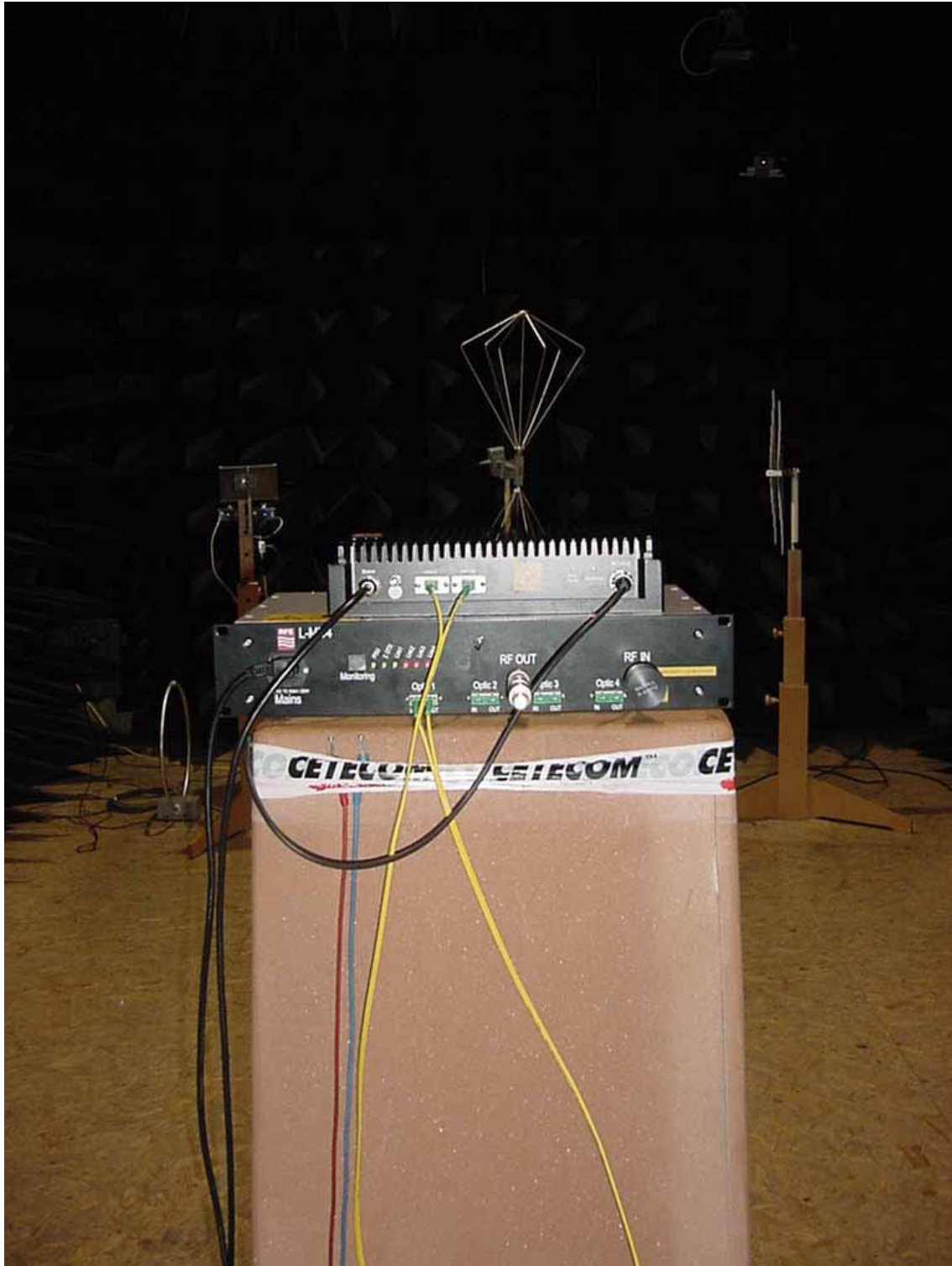
Photo 2: Radiated Emissions
